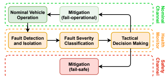
Fig. 2. Architecture approach for nominal and safety fallback functionality of an automated vehicle, including failures.
