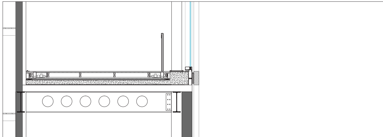
Section Fragment- Sliding
