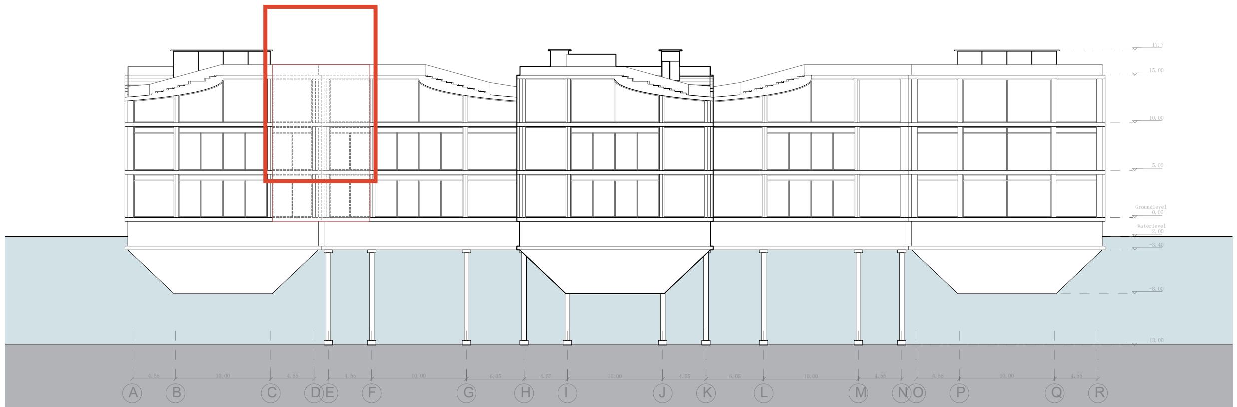
North Elevation - Cinema
