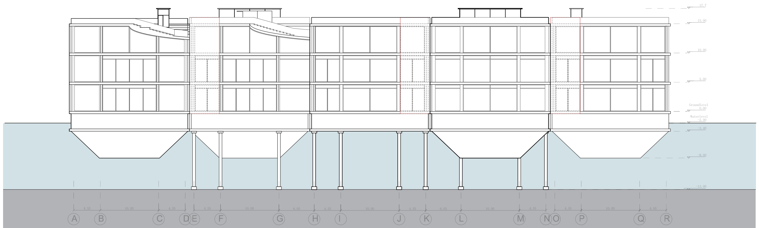
North Elevation - Theater School
