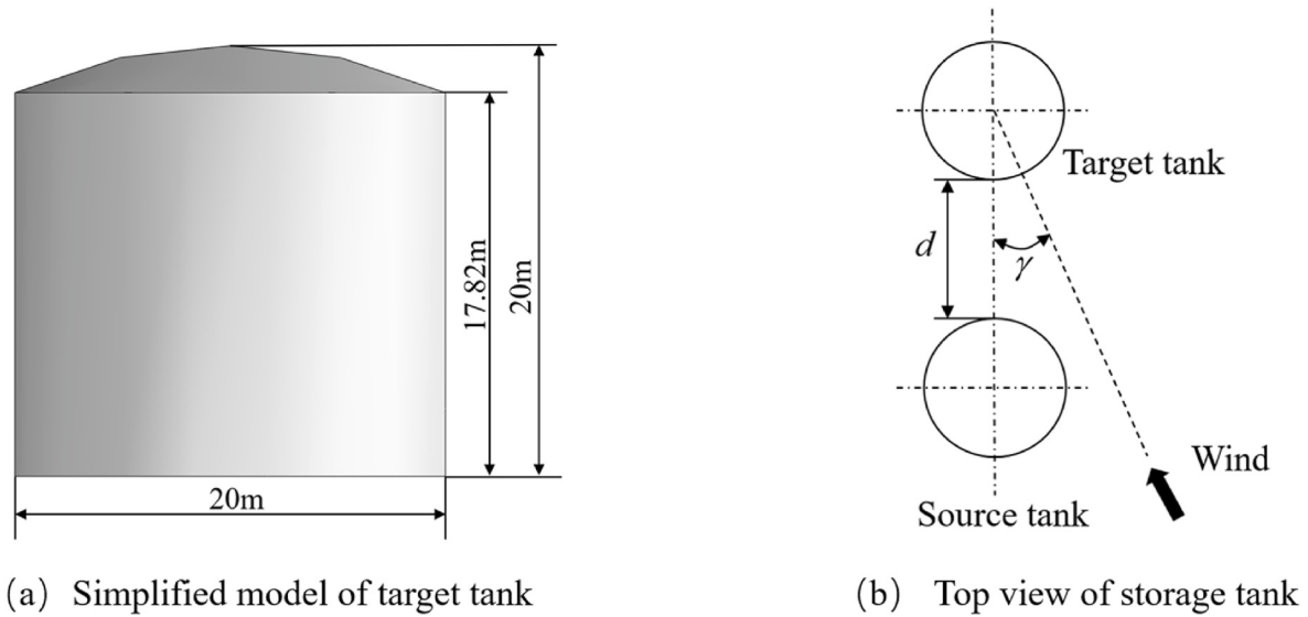
Fig. 2. Simplified model of storage tank.
