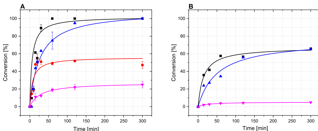
Figure 6. Application of different Thal protein concentrations ((A) 12 \mu\text{M} (1.2 mol %), (B) 2.4 \mu\text{M} (0.24 mol %)) using NADH mimics for flavin cofactor regeneration ( \blacksquare 3a, \bullet 3b, \blacktriangle 3c, \blacktriangledown 3d; 3b activity was not detected in (B)). Error bars represent the mean values \pm standard deviation from three independent reactions. Reaction conditions: 10 mM \text{Na}_2\text{HPO}_4 buffer, pH 7.4, 30 mM NaCl, 650 \text{U mL}^{-1} catalase, 10 mM NADH mimic, 1 mM tryptophan, 100 \mu\text{M} FAD, final volume 200 \mu\text{M} , shaking at 600 rpm at 25 ^\circ\text{C} .
