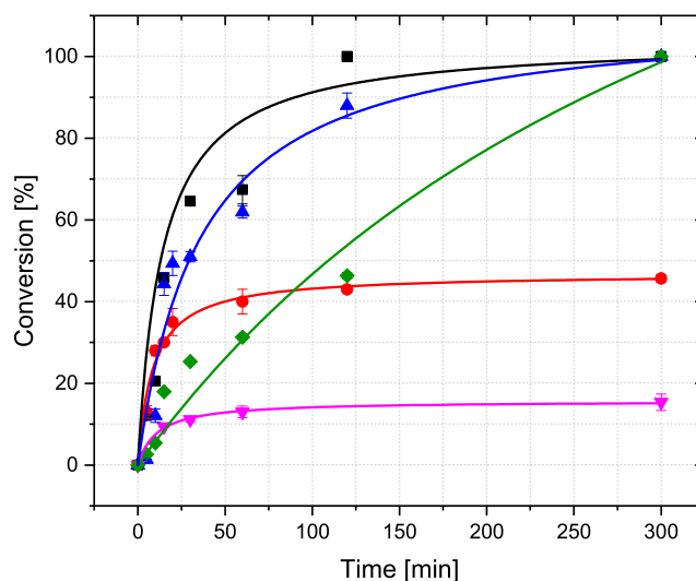
Figure 5. Screening of different NADH mimics to regenerate FADH 2 for the halogenase RebH in comparison to the conventional enzymatic regeneration system (■ 3a, ● 3b, ▲ 3c, ▼ 3d, ◆ ERS). The conversion of tryptophan was monitored with LC-MS. Reactions were done in triplicate using 1 mM tryptophan, 100 μM FAD, 1.2 mol % RebH, 650 U mL -1 catalase, and 10 mM NADH mimic or PrnF, ADH at pH 7.4 and 25 °C. In the case of the ERS, 2.5 U mL -1 flavin reductase PrnF, 1 U mL -1 alcohol dehydrogenase, 5% (v/v) isopropanol and 100 μM NAD + were used instead of the NADH mimic.
