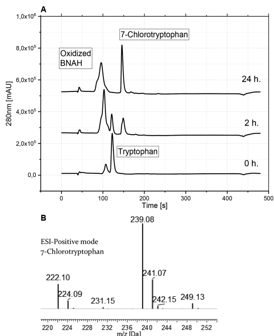
Figure 4. FADH 2 regeneration with BNAH (3a) in the enzymatic halogenation with RebH. (A) Reverse-phase high-performance liquid chromatography chromatogram. (B) Liquid chromatography-mass spectrometry (LC-MS) confirms the correct mass of the product. Reduced 3a was extracted with organic solvent before the analysis. Reaction conditions: 10 mM Na 2 HPO 4 buffer, pH 7.4, 30 mM NaCl, 650 U mL -1 catalase, 10 mM NADH mimic, 1 mM tryptophan, 100 μM FAD, 0.6 mol % (6 μM) RebH, final volume 400 μL, 600 rpm at 25 °C.
