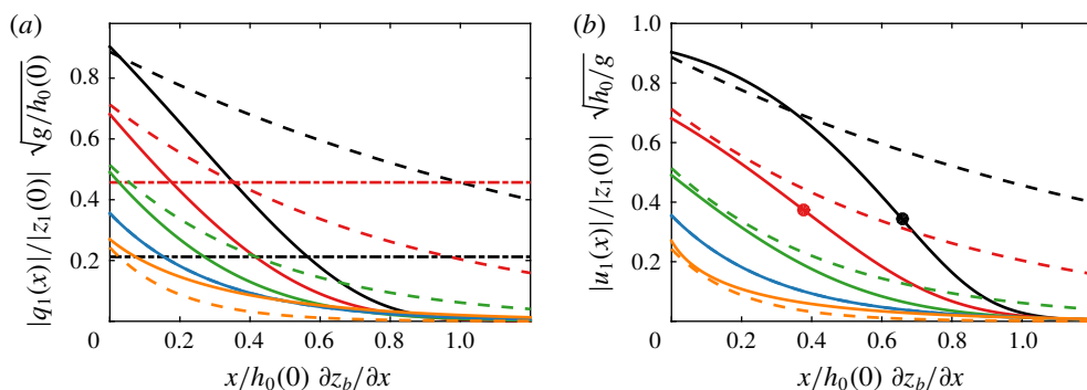
FIGURE 13. (Colour online) Magnitudes of tidal discharge (a) and tidal velocity (b), along a tidal river with a sloping bed (solid), and constant depth (dashed); river discharge indicated by dash-dotted line in (a); scenarios as in figure 8.
