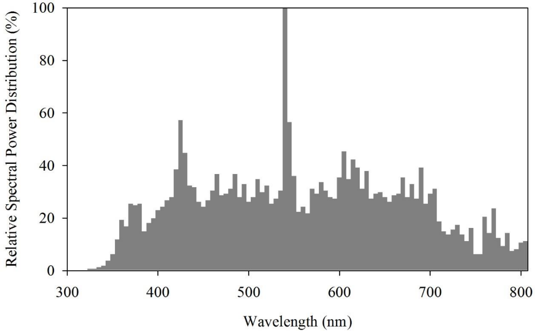
Figure 2.2 Relative spectral power distribution of the metal halide lamp used (OSRAM GmbH, Munich, Germany).
