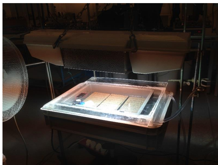
Figure 4.2 Experimental setup used for the study of the inactivation of E. coli under artificial light and dark conditions. Two such reactors were used in parallel.
