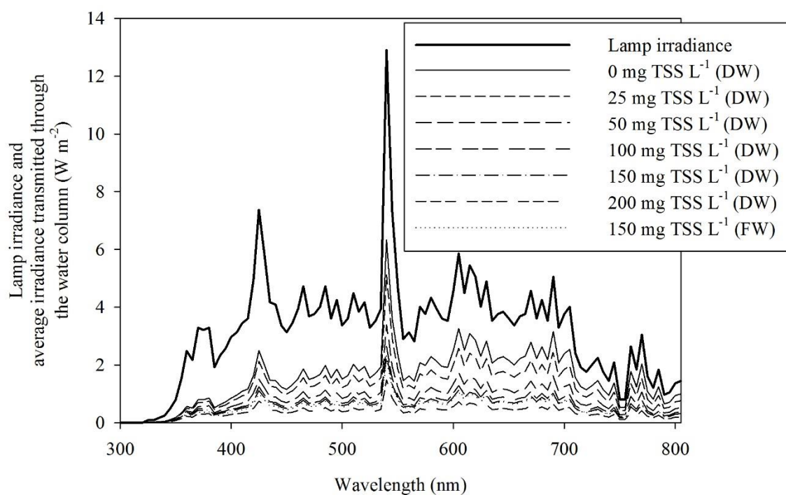
Figure 2.9 Lamp irradiance spectrum and average irradiance transmitted through the water column of demineralised water (DW) and artificial flood water (FW) with E. coli ( 7.8 \cdot 10^6 \text{ CFU.mL}^{-1} ) and different concentrations of TSS.
