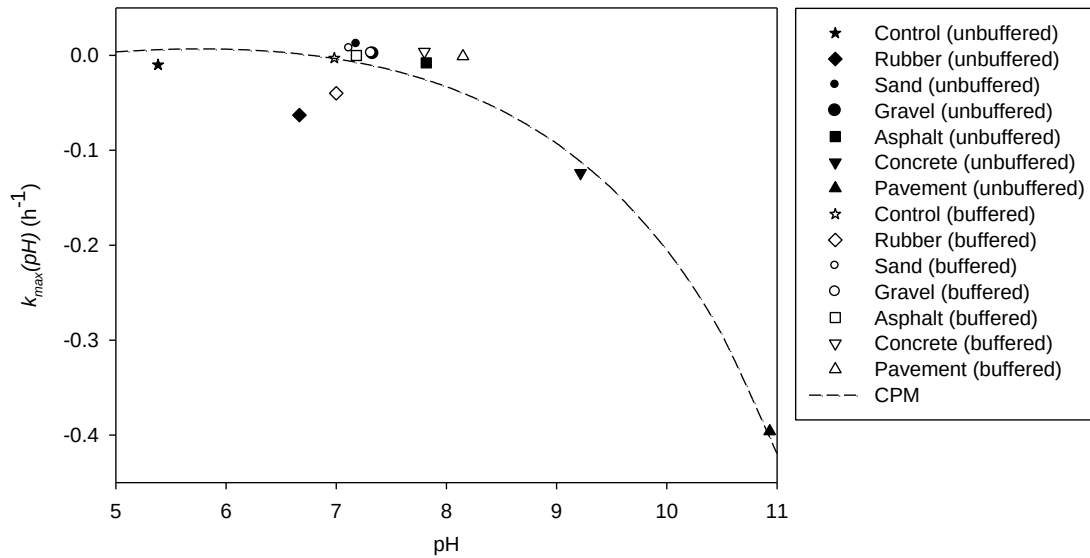
Figure 4.3 The effect of pH of water with different surface materials in batch experiments in flasks with and without the addition of HEPES, on k_{max}(pH) , of E. coli , compared to the CPM curve that best fits the data ( r^2=0.96 ). The experimental data for gravel with and without HEPES coincide. The experiments took place in room temperature of 20 °C.
