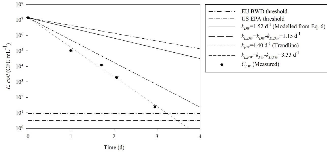
Figure 2.7 The concentration of E. coli in artificial floodwater ( C_{FW} , with inactivation rate k_{FW} ) measured in the reactor, compared to the theoretical curve for demineralised water with k_{DW}=1.52 \text{ d}^{-1} calculated from Eq. 2.7 for 150 \text{ mg TSS.L}^{-1} . The inactivation rates without the effect of dark inactivation for the two water qualities ( k_{L,FW} and k_{L,DW} , respectively) were calculated by subtracting the dark inactivation rate from the overall inactivation rate. The curves were plotted using Eq. 2.3. The threshold concentrations of E. coli according to US EPA Recreational Water Quality Criteria and EU Bathing Water Directive are also presented. Temperature was around 20^\circ\text{C} in dark conditions and increased up to 28^\circ\text{C} under exposure to light.
