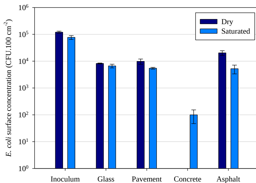
Figure 3.5 E. coli surface concentrations of the inoculum and as recovered by swabs from different surfaces, dry and saturated.
