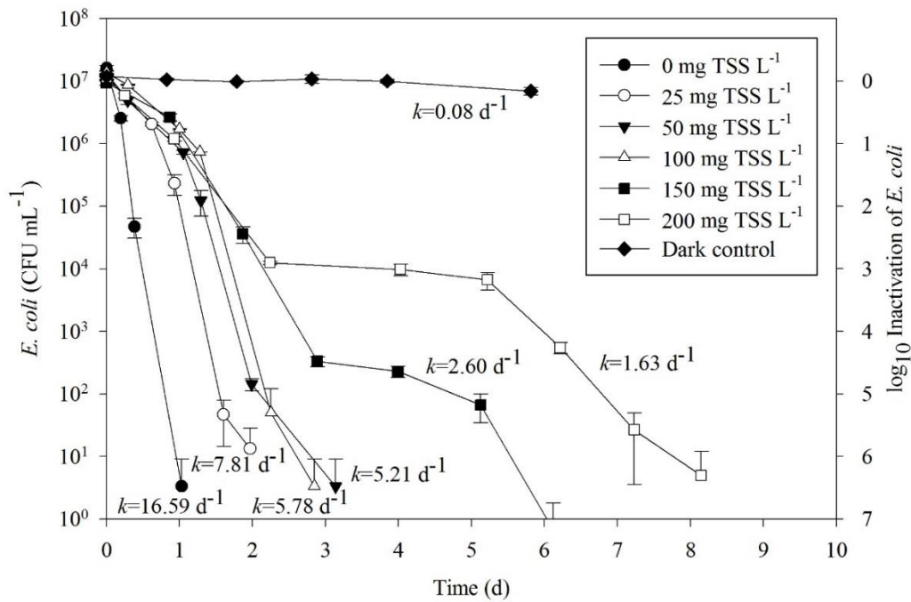
Figure 2.4 Concentration, \log_{10} inactivation and inactivation rate ( k ) of E. coli under exposure to artificial sunlight ( 320 \text{ W.m}^{-2} , 24h per day) with TSS 0, 25, 50, 100, 150 and 200 \text{mg.L}^{-1} , compared to dark control (no light and no solids). These curves correspond to the samples taken at the top of the reactor prior to filtration. Temperature fluctuated between 20^\circ\text{C} at the beginning and 28^\circ\text{C} .
