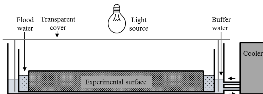
Figure 4.1. Schematic representation of a reactor exposed to artificial light. Two such reactors were used in parallel.
