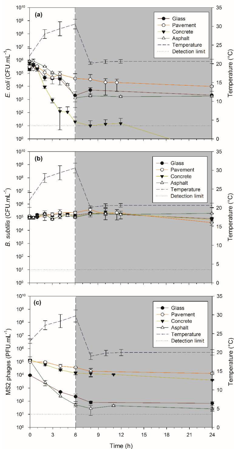
Figure 5.4 Inactivation of E. coli (a), B. subtilis (b) and MS2 bacteriophages (c) on different surfaces. The white area represents the light phase and the grey area represents the dark phase.
