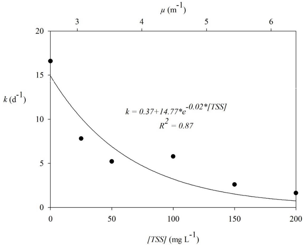
Figure 2.5 The effect of TSS concentration ( \text{mg.L}^{-1} , lower horizontal axis) and of light attenuation coefficient \mu ( \text{m}^{-1} , upper horizontal axis) on inactivation rate k ( \text{d}^{-1} ) of E. coli measured in the reactor under continuous exposure to artificial sunlight ( 320 \text{ W.m}^{-2} ). The coefficient \mu was calculated based on Equation 2.5.
