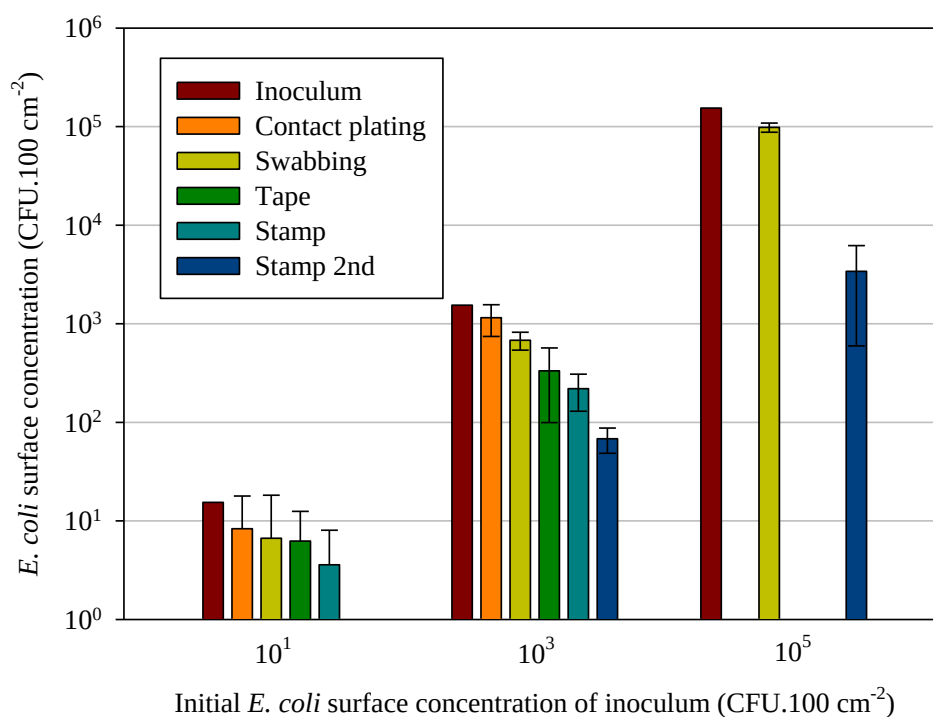
Figure 3.4 E. coli surface concentrations recovered with different methods from a glass surface compared to the surface concentration of the inoculum initially spread over of around 10 1 (left cluster), 10 3 (central cluster) and 10 5 (right cluster) CFU.100 cm -2 .
