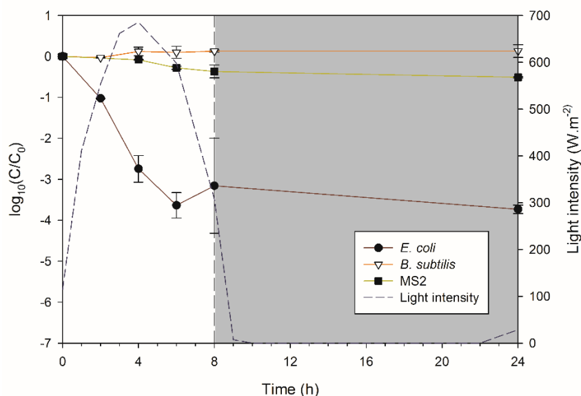
Figure 5.5 Inactivation of E. coli , B. subtilis and MS2 on pavement under natural sunlight (white area) and dark (grey area).
