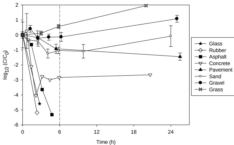
Figure 4.5 Inactivation of E. coli on different surfaces, recovered by swabbing. The vertical line at 6 h signifies the transition from the light to the dark phase. The detection limit corresponds to \log_{10}(C/C_0) = -4 .
