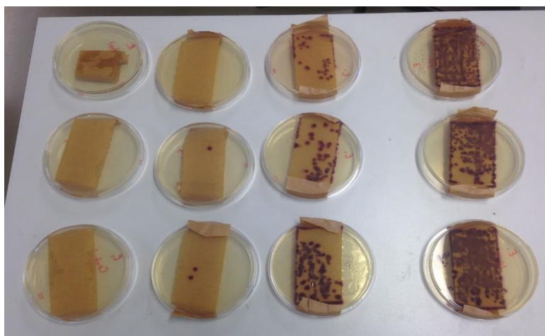
Figure 3.2 Petri dishes with adhesive tape on CCA medium after sampling and incubation. The first column is the control and the other columns contain different concentrations of E. coli. Sampling was performed in triplicate (three rows).
