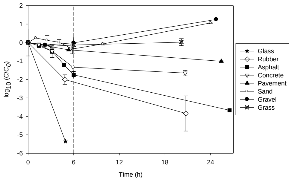
Figure 4.4 Inactivation of E. coli in water samples around different flooded surfaces. The vertical line at 6 h signifies the transition from the light to the dark phase. The detection limit corresponds to \log_{10}(C/C_0) = -4 .
