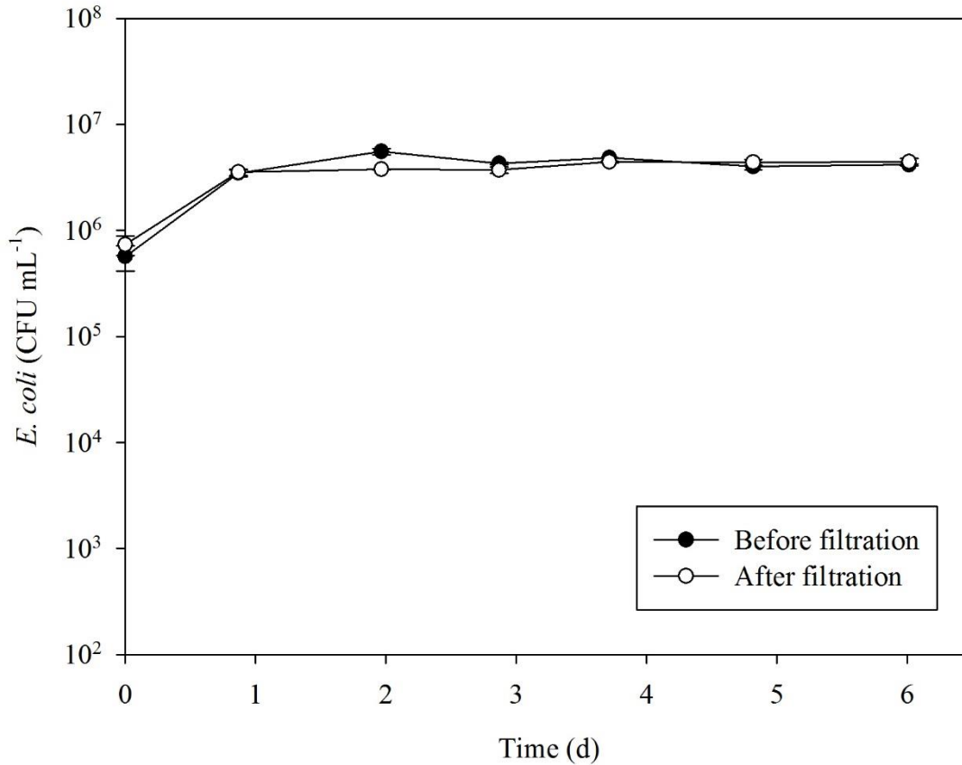
Figure 2.6 The concentration of E. coli in demineralised water with 200 mg TSS.L -1 , before and after filtration (11 \mu m) in a batch experiment in Erlenmeyer flasks.
