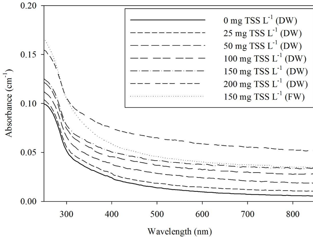
Figure 2.8 Absorbance spectra of demineralised water (DW) and artificial flood water (FW) with E. coli ( 7.8 \cdot 10^6 \text{ CFU.mL}^{-1} ) and different concentrations of TSS.
