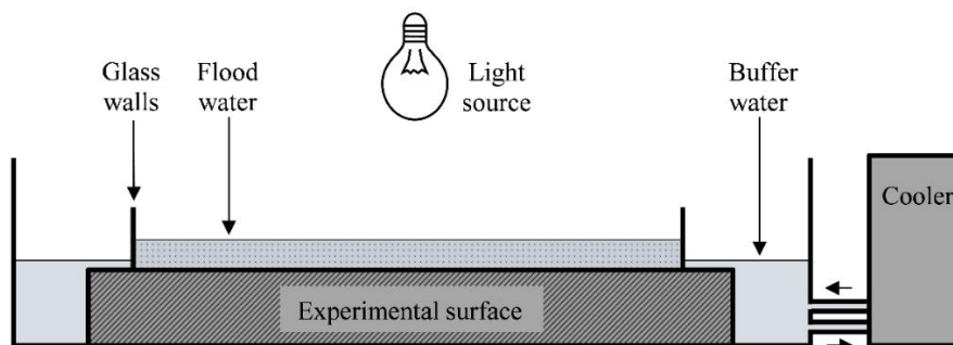
Figure 5.1. Schematic representation of a reactor exposed to artificial light. Two such reactors were used in parallel. In the experiments under real sunlight the cooler was not used.
