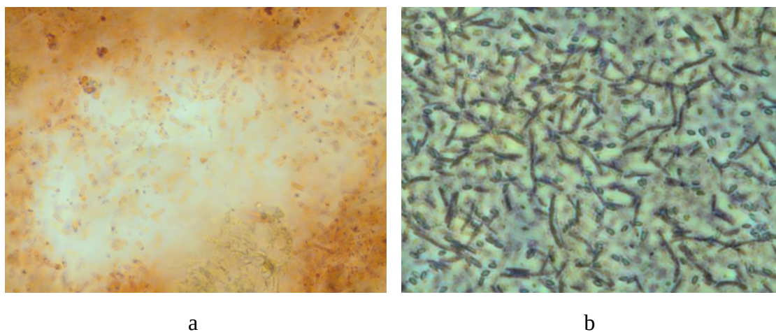
Figure 5.3. B. subtilis spores under 100x magnification. Before pasteurization (a), the spores can be seen inside vegetative cells. After pasteurization and sonication (b), spores (green in colour) are released from inactivated cells (brown in colour).
