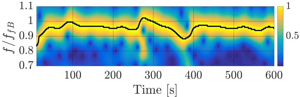
Figure 7: S-transform of the OWT response for the load time history in Figure 3(b). All frequency values are normalized with respect to the fixed-base natural frequency f_{FB} of the OWT. The colorbar indicates the magnitude of all harmonics, the thick black line underlines the evolution of the peak frequency.
