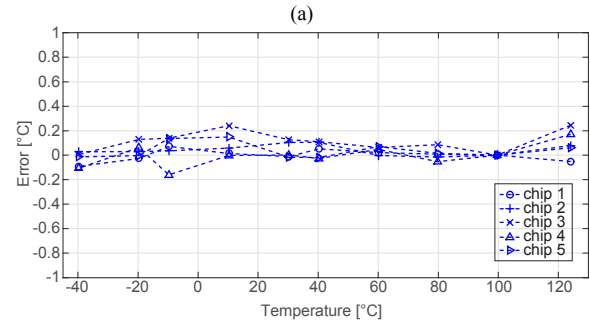
Fig. 14. Measured temperature error of the algorithmic temperature sensor (a) without and (b) with correction for leakage and series resistance
