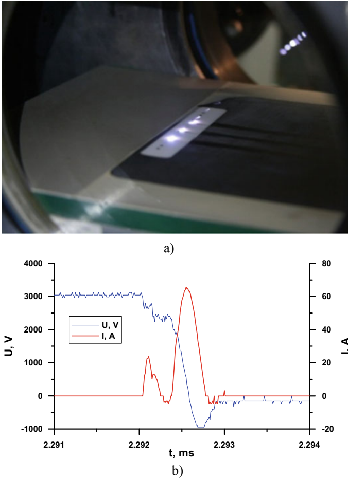
Fig. 8 a Model with spark discharge actuator and b voltage and current oscillograms
