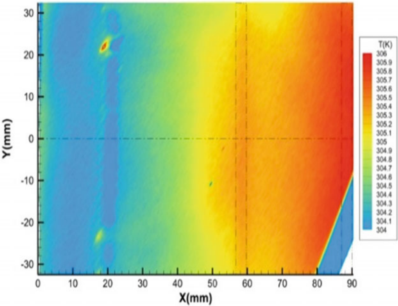
a) - control device at X_{d1} location
