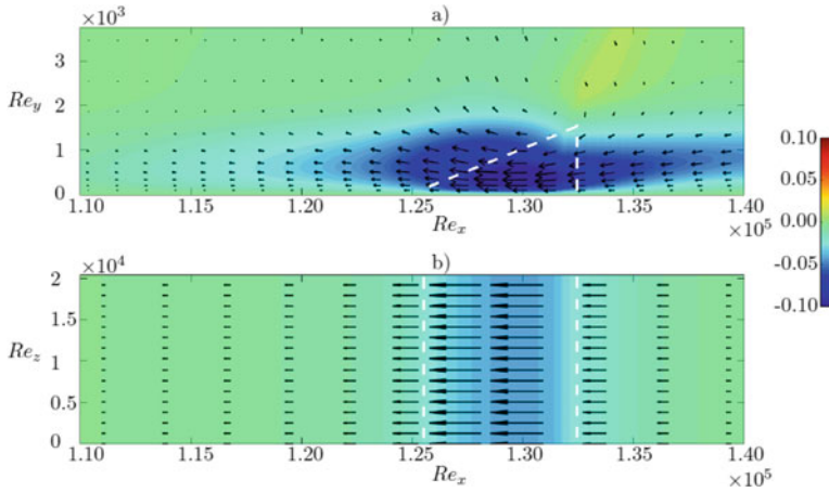
Fig. 25 Induced streamwise velocity vectors superimposed onto the induced streamwise velocity contours on a a x-y plane at z = L_z/4 and b a x-z plane at y = 0.1 \delta_{1,0} for counter-flow actuation with straight-edged electrodes and no electric field spanwise variation (case 5). The DBD position and shape is indicated by the white dashed lines
