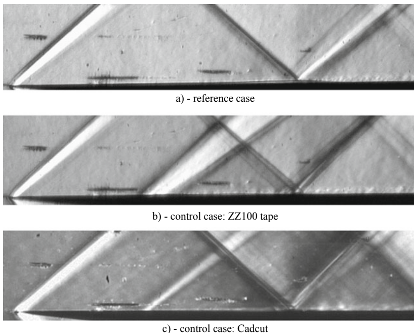
Fig. 57 Schlieren visualizations (devices at X_{d1} location)
