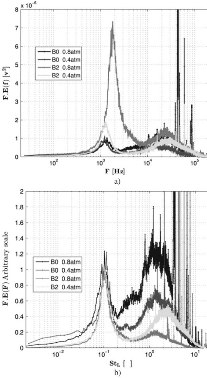
Fig. 3 Pre multiplied PSD, natural (B0) and tripped (B2) boundary layer, \Theta_3 flow deviation, at P_{gen} = 0.4 atm and P_{gen} = 0.8 atm total pressure. a: pre-multiplied spectra vs frequency F , b: normalized pre-multiplied spectra vs Strouhal number St_L = FL/U_1
