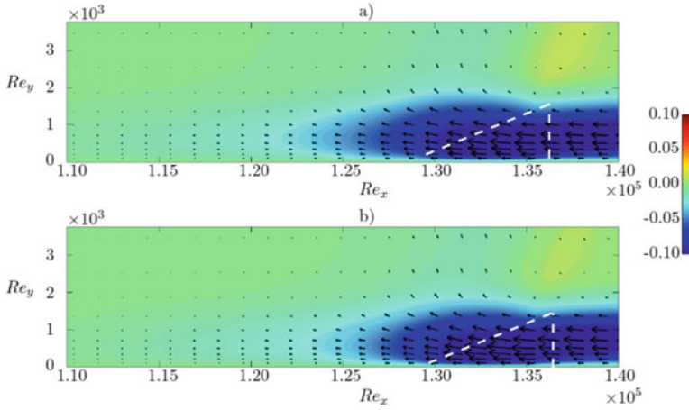
Fig. 26 Induced streamwise velocity vectors superimposed onto the induced stream-wise velocity contours on an x-y plane at z = L_z/4 for counter-flow actuation with a serpentine (case 6) and b horseshoe (case 9) electrodes. The DBD position and shape is indicated by the white dashed lines
