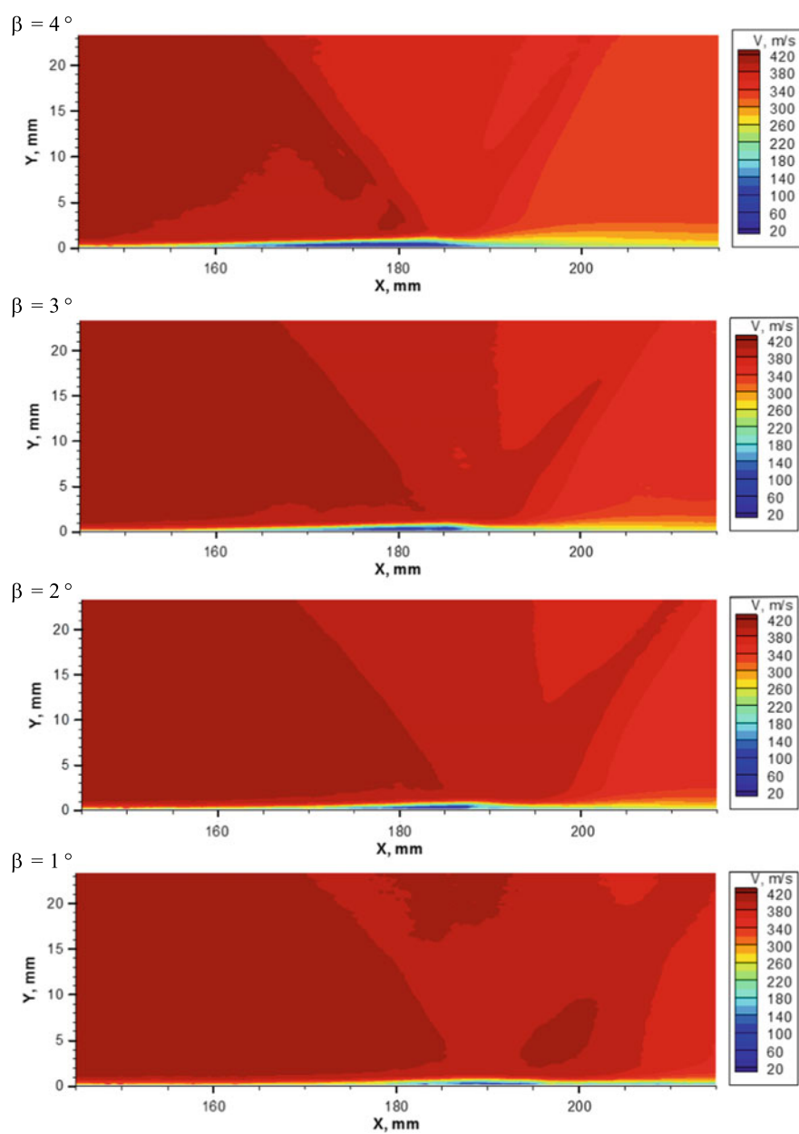
Fig. 53 Velocity fields (transitional case, L = 200 mm, Re_1 = 10.9 \times 10^6 1/m)
