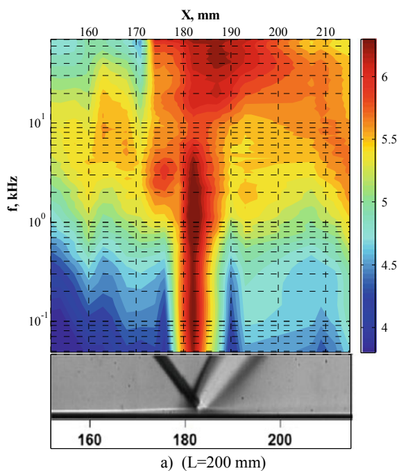
Fig. 55 Spectrogram of wall pressure pulsations for laminar test case ( P_0 = 0.7 bar)
