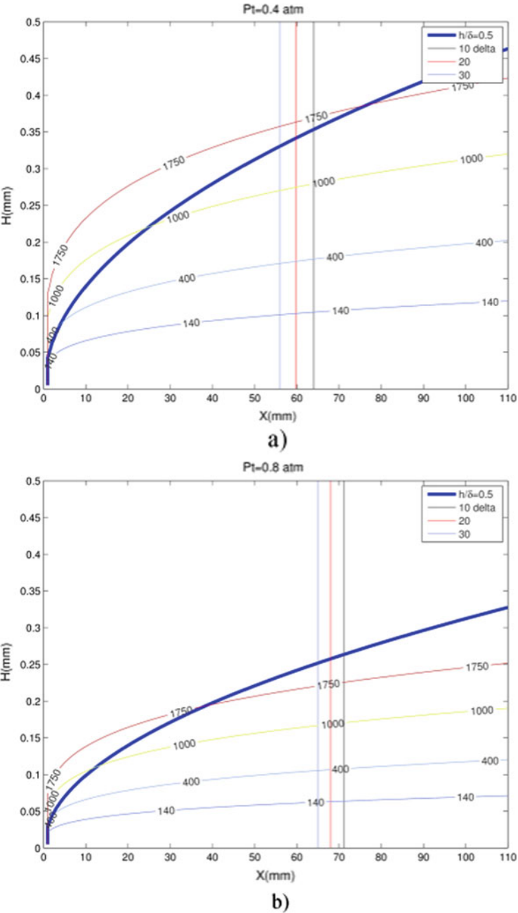
Fig. 51 Characteristic immersed Reynolds numbers. a P_0 = 0.4 \text{ atm} ; b P_0 = 0.8 \text{ atm}
