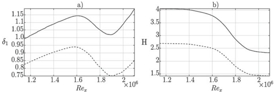
Fig. 70 Time- and span-averaged displacement thickness (a) and shape factor (b) distributions calculated with the incompressible (dashed lines) and compressible (solid lines) formulations
