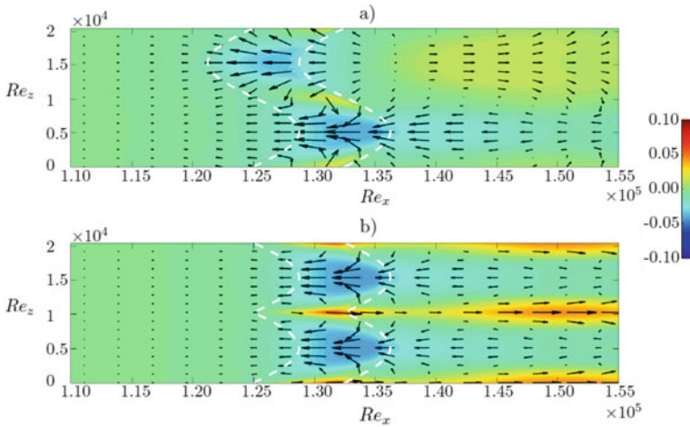
Fig. 27 Induced streamwise velocity vectors superimposed onto the induced streamwise velocity contours on an x-z plane at y = 0.1 \delta_{1,0} for counter-flow actuation with a serpentine (case 6) and b horseshoe (case 9) electrodes. The DBD position and shape is indicated by the white dashed lines
