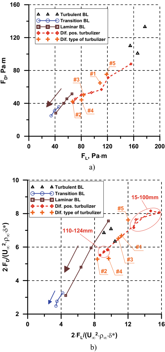
Fig. 56 Dimension (a) and dimensionless (b) values of total pressure loss vs the increase of wall pressure on the model
