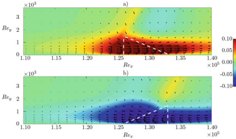
Fig. 23 Induced streamwise velocity vectors superimposed onto the induced streamwise velocity contours on an x-y plane at z = L_z/4 for a co-flow (case 2) and b counter-flow (case 4) actuations with straight-edged electrodes. The DBD position and shape is indicated by the white dashed lines
