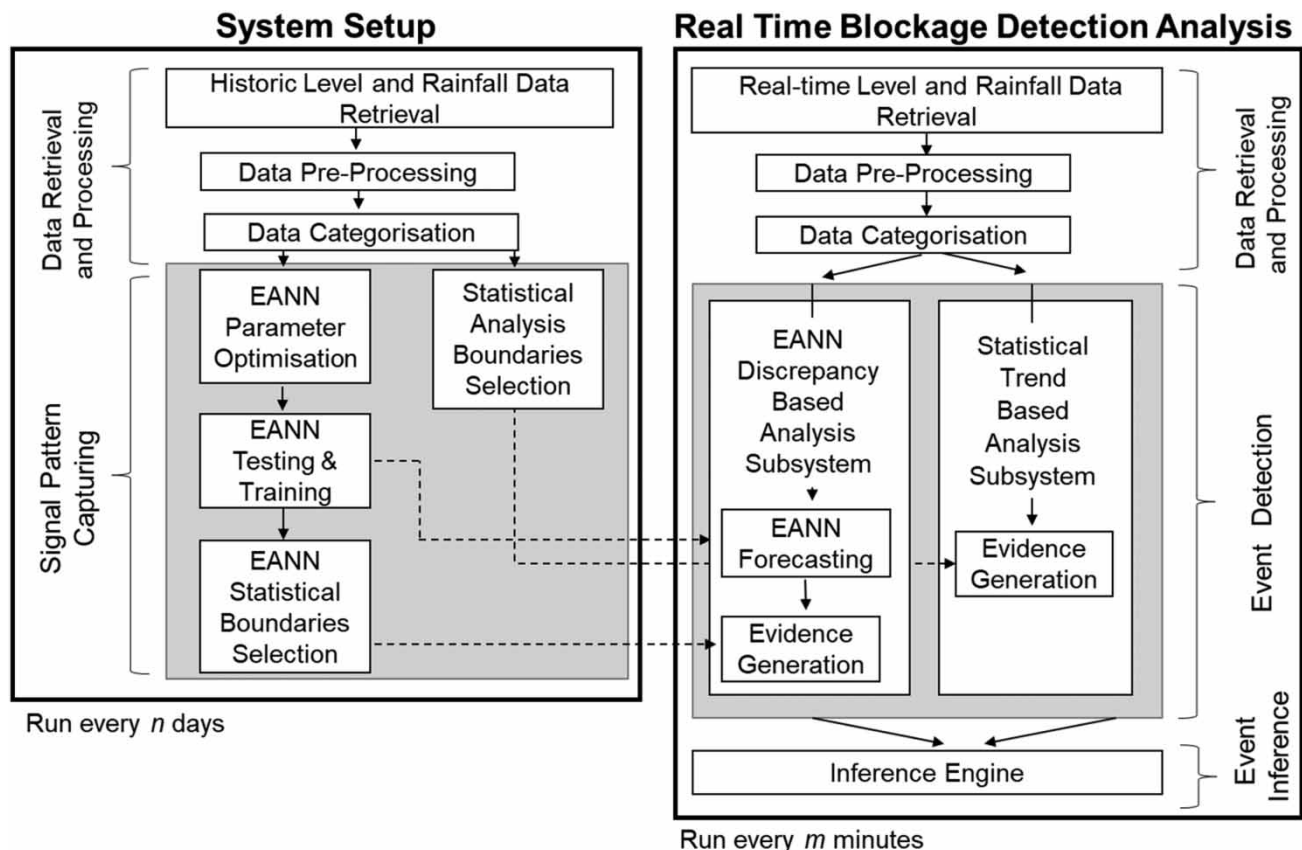
Figure 1 | Diagrammatic representation of the EDS methodology (left figure shows the offline system set-up and the right one shows the online application in near real-time).
