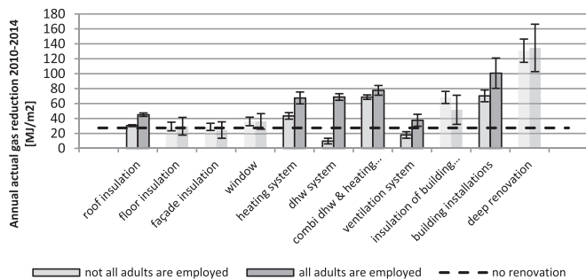
Fig. 6. Difference in energy saving (corrected for degree days) for households where all occupants have jobs and those in which not all occupants have jobs – insignificant measures are shown transparent.
