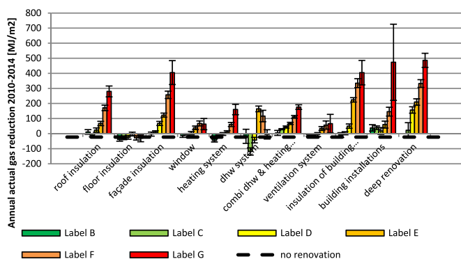
Fig. 9. Average energy saving gap per energy label of the building prior to renovation for every type of thermal renovation.
