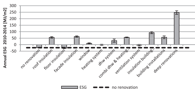
Fig. 8. Average energy saving gap per thermal renovation measure.
