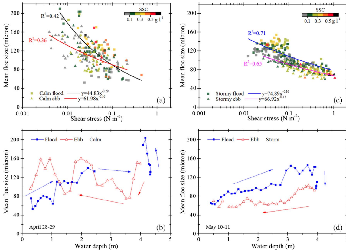
Fig. 8. (a)(c) Variation of mean floc size and shear stress under calm flood/ebb and stormy flood/ebb conditions, respectively; (b)(d) Typical variation of mean floc size with water depth in a tidal cycle under calm and stormy conditions on April 28–29 and May 10–11, respectively. In (a) and (c), solid lines are the regression results, and colour bar indicates corresponding suspended sediment concentration SSC. In (b) and (d), blue and red symbols represent flood and ebb tide, respectively. (For interpretation of the references to colour in this figure legend, the reader is referred to the web version of this article.)
