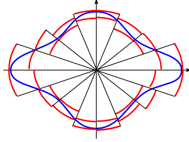
Figure 5.9: Spherical inner- and outer-approximations for each conic section of \underline{M}_{\underline{\tau}_\star} .
