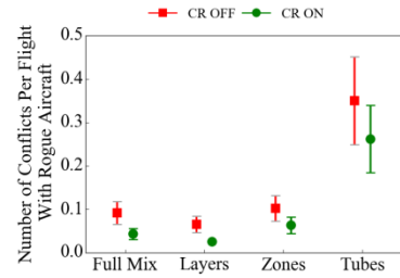
Figure 14b: Effect of Conflict Resolution (CR)
