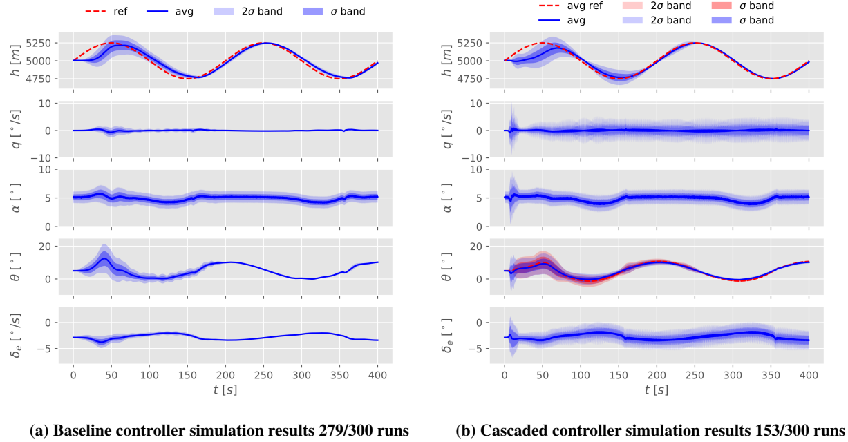
Fig. 7 Comparison of converged runs under measurement noise
