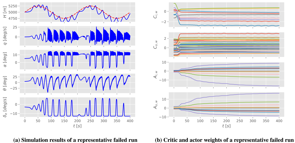
Fig. 6 Representative failed run of a baseline controller under perfect conditions
