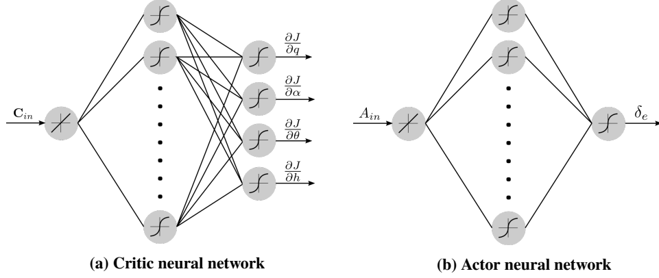
Fig. 3 Critic and actor structure
