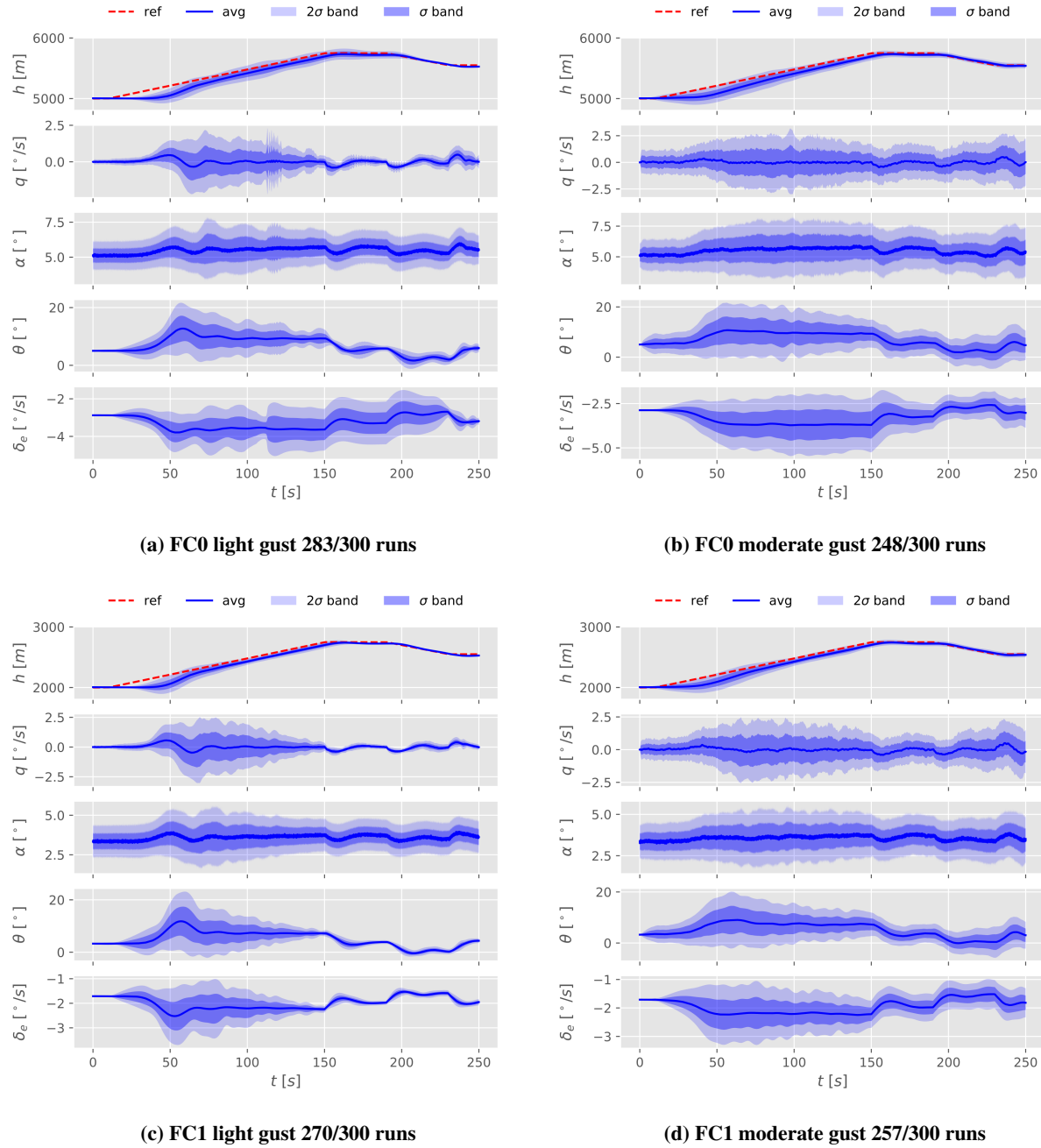
Fig. 8 Simulation results obtained with measurement noise and varying gust conditions for FC0 and FC1
