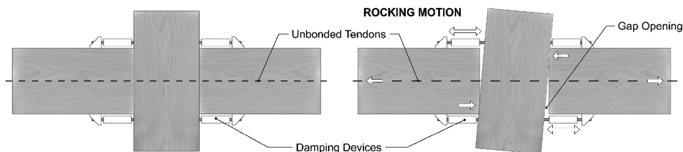
FIGURE 1 Hybrid post-tensioned dissipative connection for timber elements.
