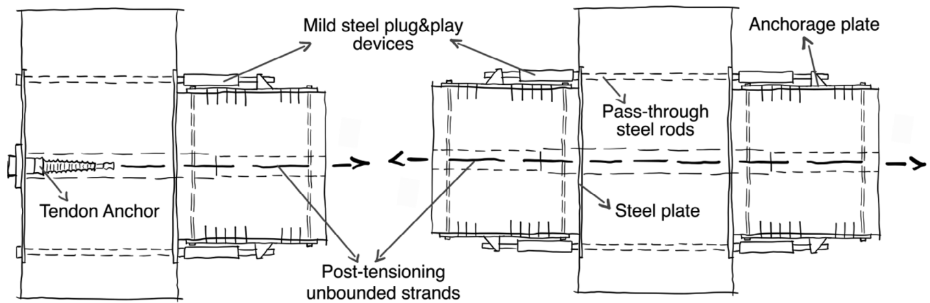
FIGURE 8 A sketch of the connection details for both external and internal beam-column joints.
