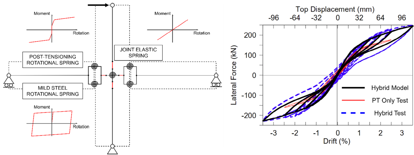
FIGURE 11 Details of the numerical modelling of the specimen tested by Iqbal et al. 32 (A) and numerical vs. experimental comparison (B).
