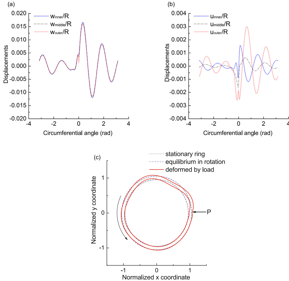
Fig. 11. High-order model, displacements under a harmonic load, \bar{v} = 0.3, \bar{k}_r = 0.01, \bar{k}_c = 0.1, \zeta = 0.002, \bar{\Omega}_f = 0.15 : (a) Radial displacement; (b) Circumferential displacement; (c) Ring deformation. The ring deformation is scaled by 5.
