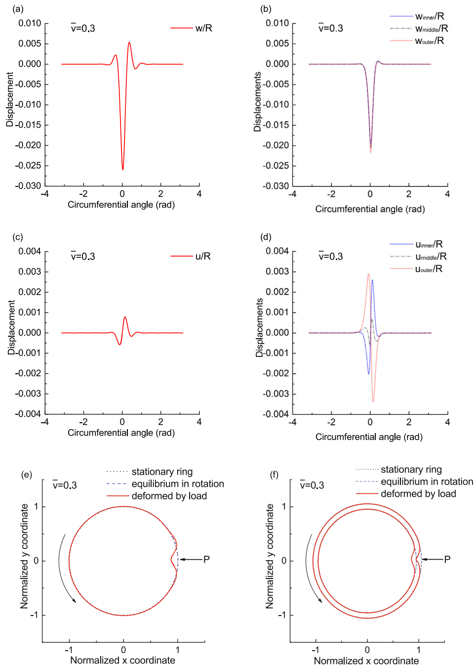
Fig. 8. Responses predicted using the classical (left) and high-order (right) models for \bar{\nu} = 0.3 , \bar{k}_r = 0.01 , \bar{k}_c = 0.1 : (a) and (b) Radial displacements; (c) and (d) Circumferential displacements; (e) and (f) Ring deformation. The ring deformations are scaled by 5.
