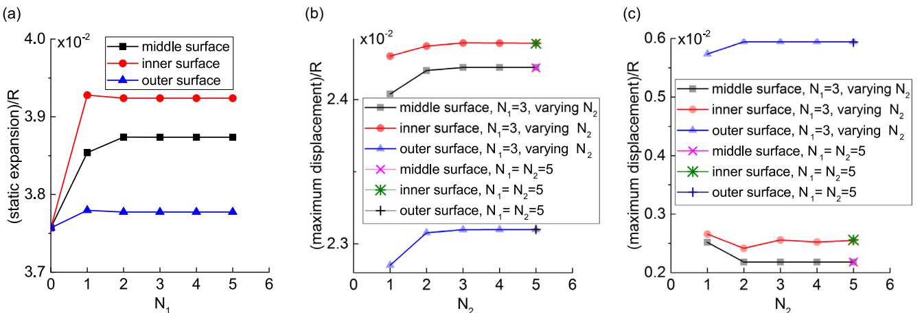
Fig. 12. Convergence check of the displacements at different positions of the ring for \bar{v} = 0.7, \bar{k}_r = 0.01, \bar{k}_c = 0.1, \zeta = 0.002 : (a) Static radial expansion due to rotation; (b) Radial displacement; (c) Circumferential displacement.
