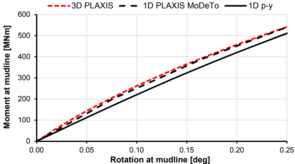
Fig. 4. Moment versus rotation at mudline for the design model
