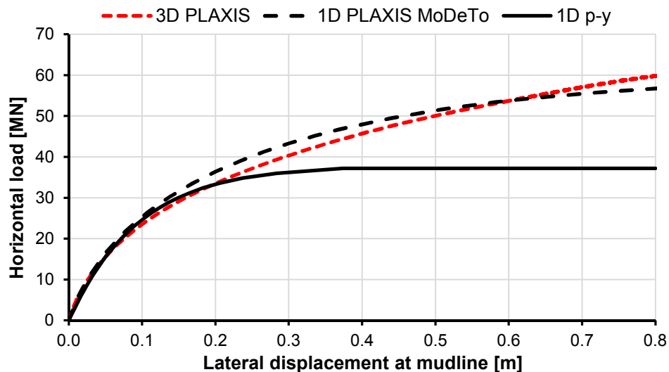
Fig. 3. Horizontal load versus latera displacement at mudline for the design model
