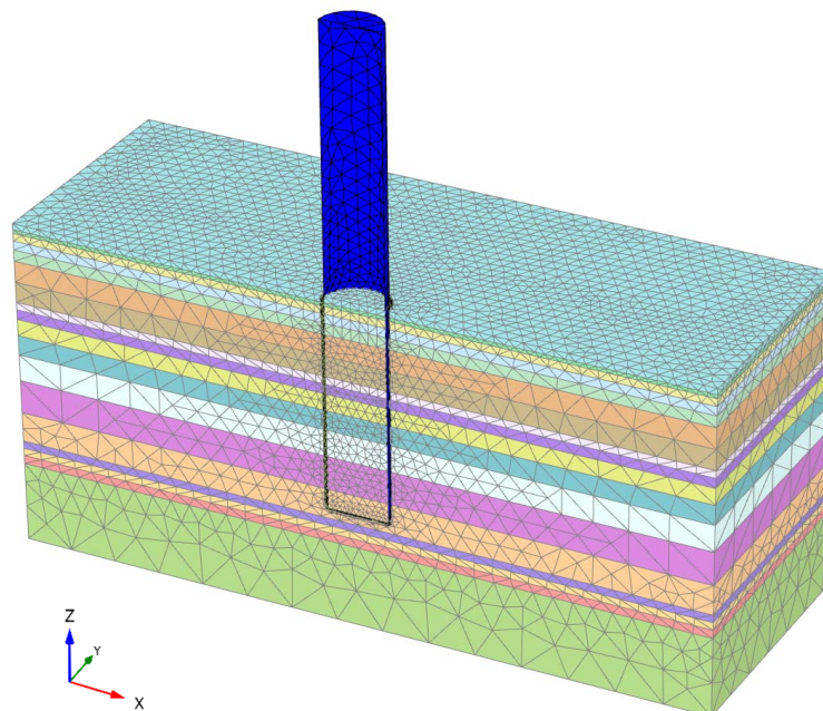
Fig. 1. Calibration model CM5
