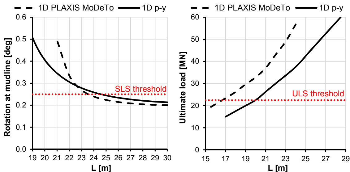
Fig. 2. Penetration depth analysis for the SLS (left) and ULS (right) design criteria
