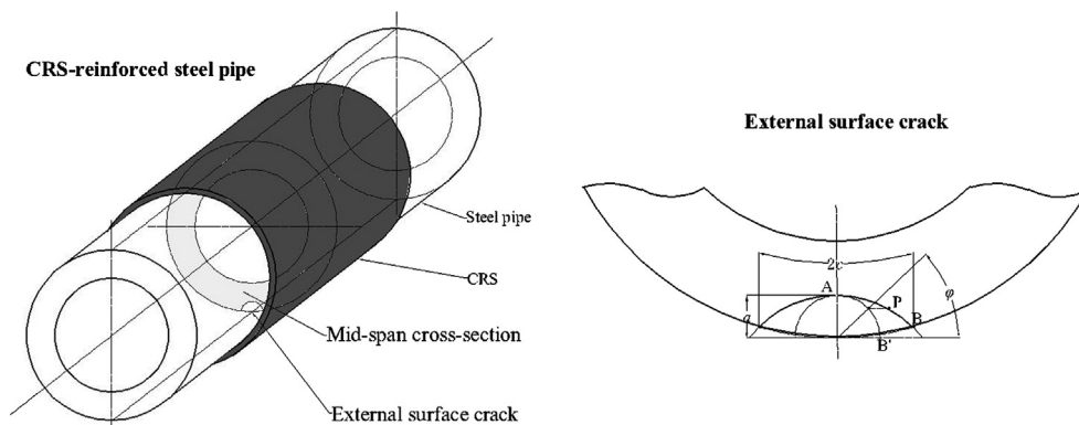
Fig. 1. The sketch diagram of the CRS reinforced surface cracked pipe specimens.
