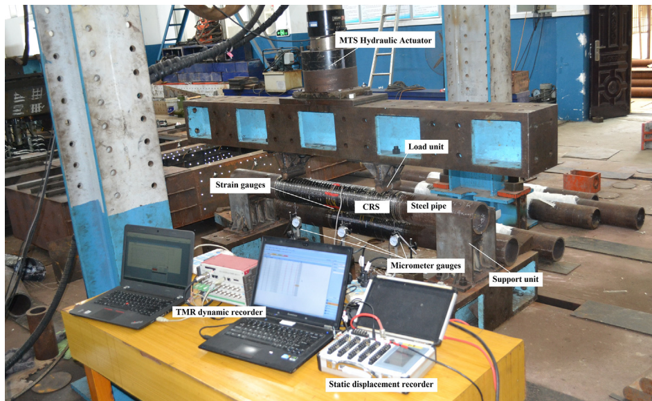
Fig. 6. Specimen and instruments installation.
