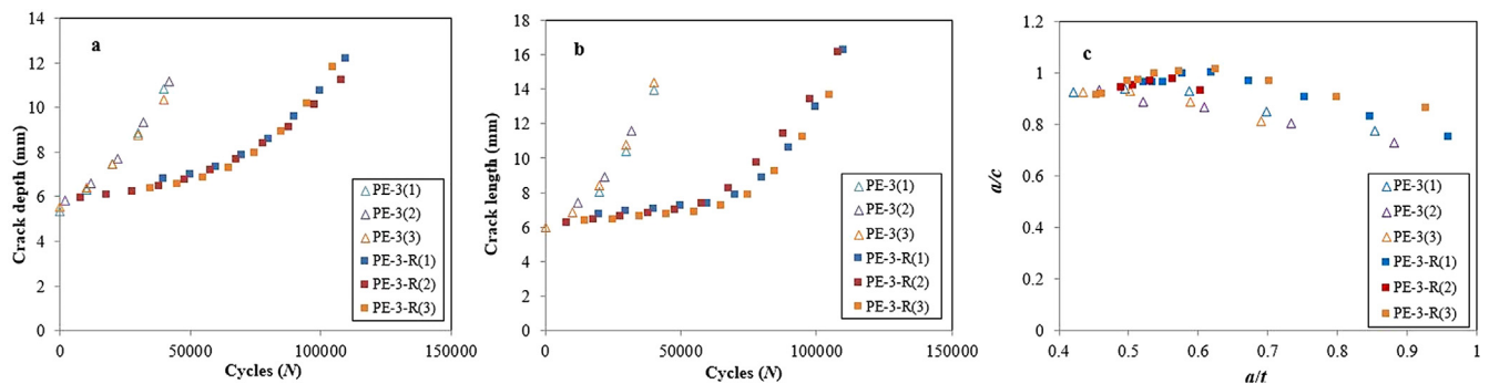
Fig. 13. The experimental results of PE-3 and PE-3-R of using the default reinforcement scheme: a) crack growth along depth direction; b) crack growth along length direction; c) aspect ratio variation: a/c versus a/t curves.
