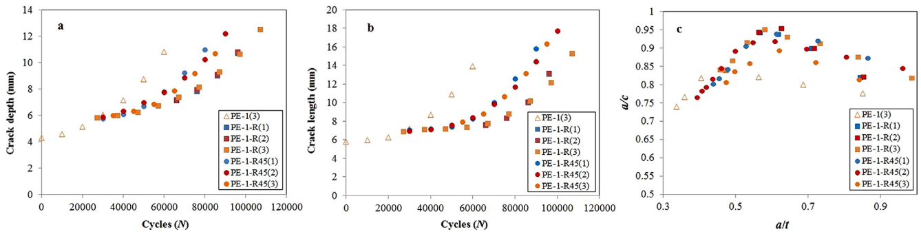
Fig. 16. The experimental result comparison between using L-L-L-H CFRP wrapping (PE-1-R) and inversely diagonal wrapping (PE-1-R45) method: a) crack growth along depth direction; b) crack growth along length direction; c) aspect ratio variation: a/c versus a/t curves.
