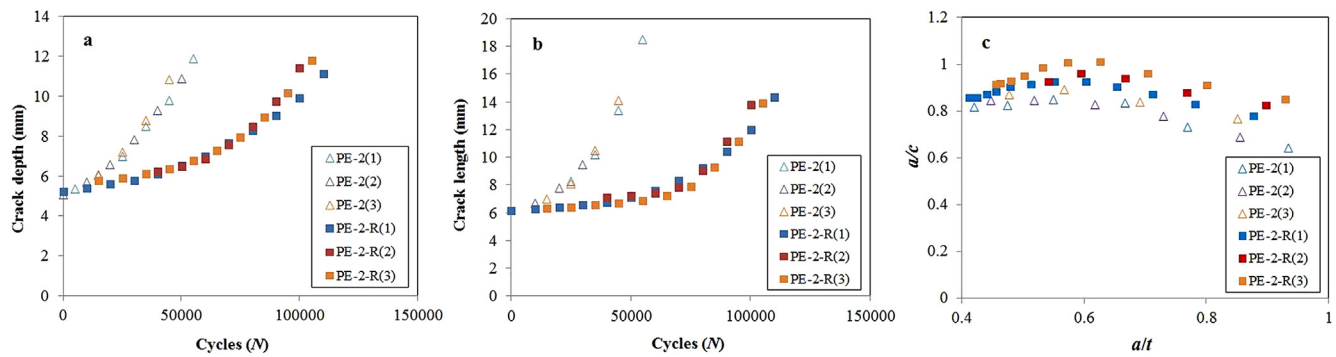
Fig. 12. The experimental results of PE-2 and PE-2-R of using the default reinforcement scheme: a) crack growth along depth direction; b) crack growth along length direction; c) aspect ratio variation: a/c versus a/t curves.
