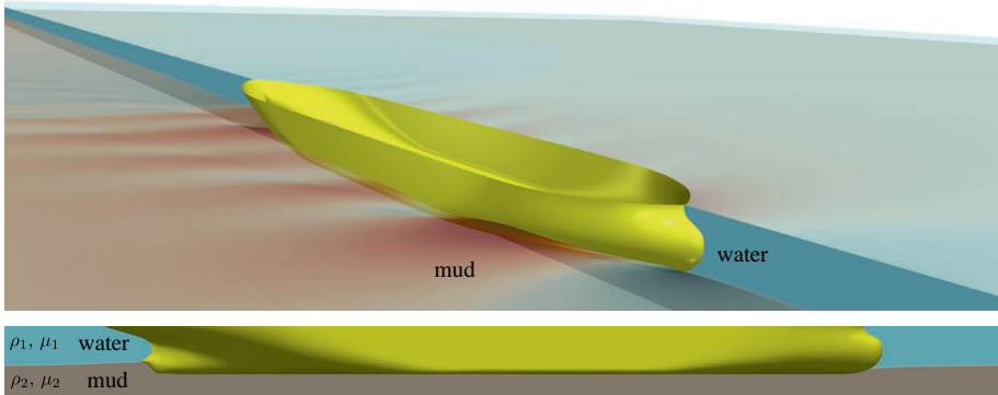
Figure 2.1: Example of a typical scenario simulated with CFD. The free-surface waves are neglected, while mud and water are assumed to be immiscible.
