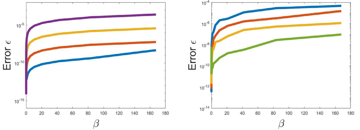
Fig. 3. The behaviour of the error \varepsilon as a function of \beta for \alpha_1 = \alpha_2 = 1 . Each curve represents a number of finite element nodes: 48, 192, 768 and 3072 nodes (from top to bottom). Left: equidistant mesh; Right: one sample with a randomised mesh.
