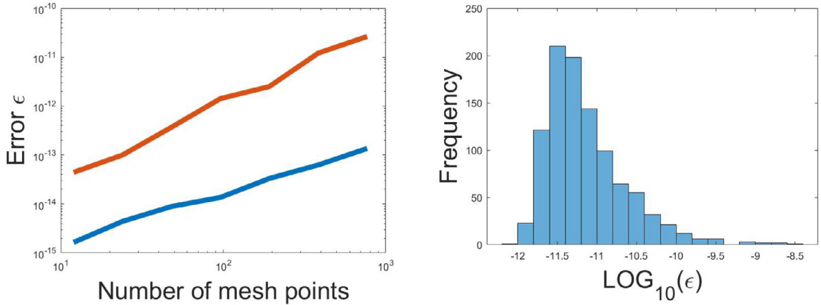
Fig. 2. Left: the behaviour of the error \varepsilon as a function of the number of nodal points for \alpha_1 = \alpha_2 = 1 . The upper red curve is the arithmetic mean of the error of 1000 samples with randomised meshes, the lower blue curve is for equidistant meshes; Right: histogram of the logarithm with basis 10 of the error for randomised meshes after 1000 samples with a mesh of 768 nodes. (For interpretation of the references to colour in this figure legend, the reader is referred to the web version of this article.)
