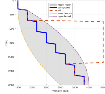
Figure 4: Bounds on the sediment velocity
