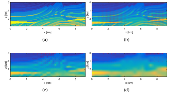
Figure 2: An example of bilinear interpolation. The less nodes, from (a) to (d), the smoother the representation of the model.
