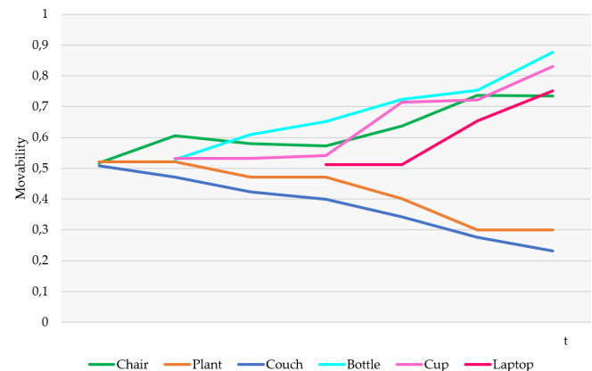
Fig. 7. Evolution of the movability for each object class during the mapping sessions.
