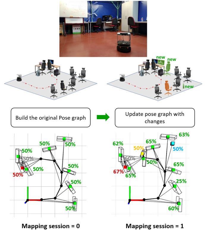
Fig. 1. Proof of concept of the dynamic mapping method in an indoor environment. First, the original object-based pose graph is built (7 chairs, 1 computer and 1 backpack were mapped). For the adaptation of the map, one chair was moved and a bottle and a screen were added. The map adapted to the changes adding the new objects and increasing or decreasing the probabilities of the old ones.
