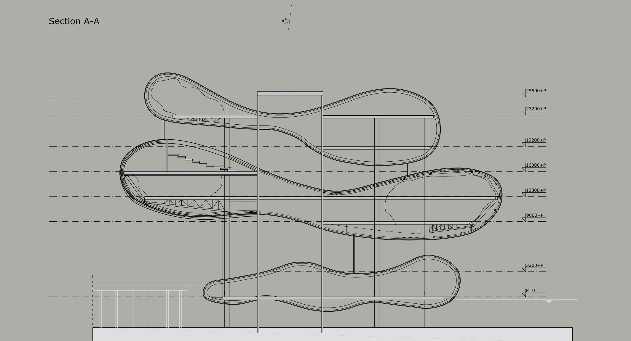
Cross Section
