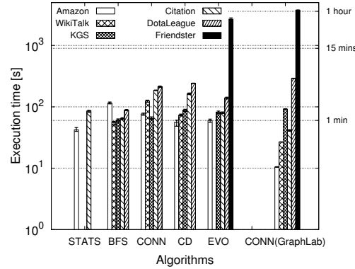
Figure 3.3: The execution time of all algorithms for all datasets running on Giraph, and for CONN running on GraphLab (right-most bars).
