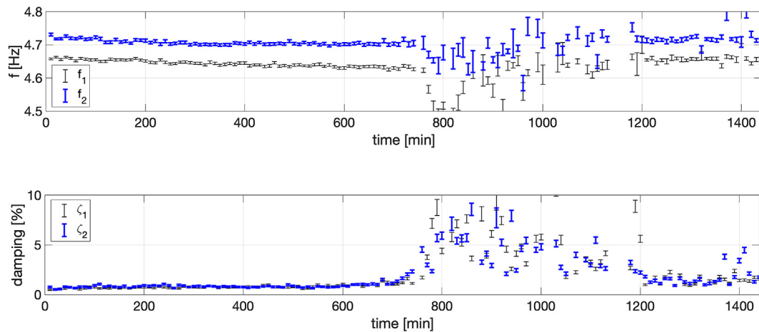
Fig. 16. Wolf Rock monitoring. Frequency estimation (upper) and damping estimation (lower) from application of BAYOMA to data of Fig. 16.
