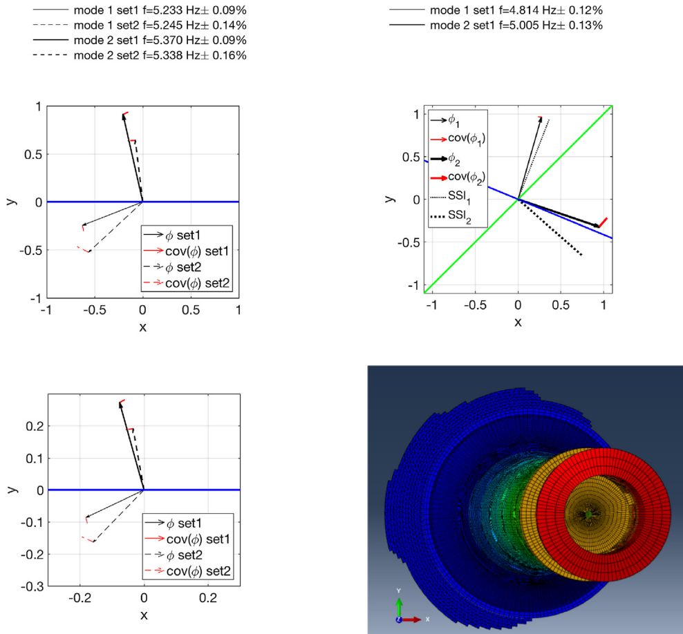
Fig. 11. Left column Dubh Artach level 7 (upper) and level 3 (lower); x axis (blue line) is aligned with openings (windows, doors). Right column Fastnet; x axis aligns with entrance, green line is North-South axis, blue line is x axis of FEM. FEM second mode, along the model axes shown bottom right. (For interpretation of the references to colour in this figure legend, the reader is referred to the web version of this article.)
