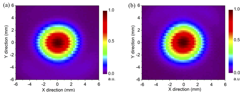
Fig. 6. (a) Intensity image plot of the input beam. (b) Intensity image plot of the output beam from the lens system without the gold layer. The color indicates relative intensity.
