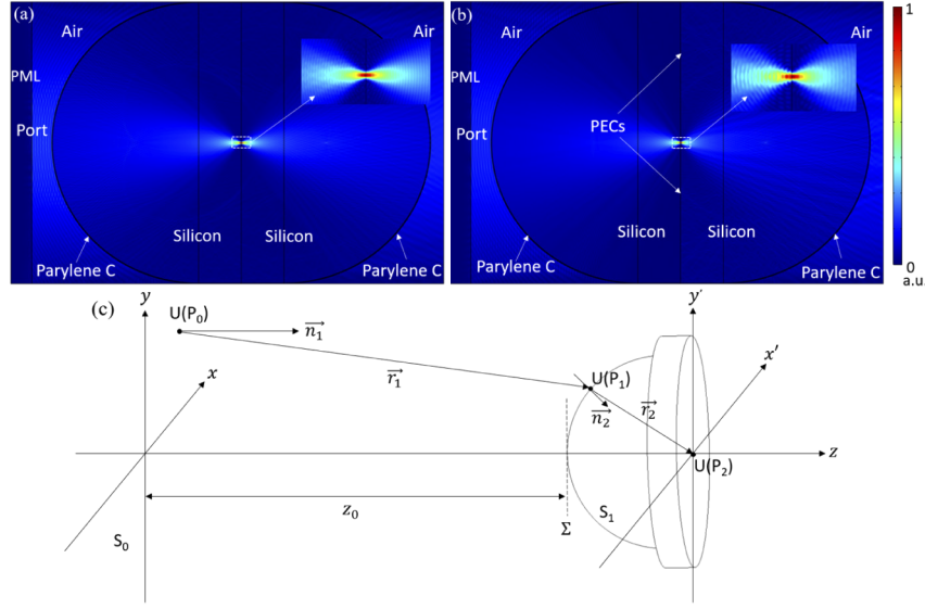
Fig. 2. (a) 2D model of the B2B lens system without apertures in simulation. Different colors indicate the electric field distribution. The inset is the field distribution around the focal point of the lens system. (b) 2D model of the B2B lens system with an aperture in simulation. (c) Schematic of field propagation from the xy plane to the x'y' plane.
