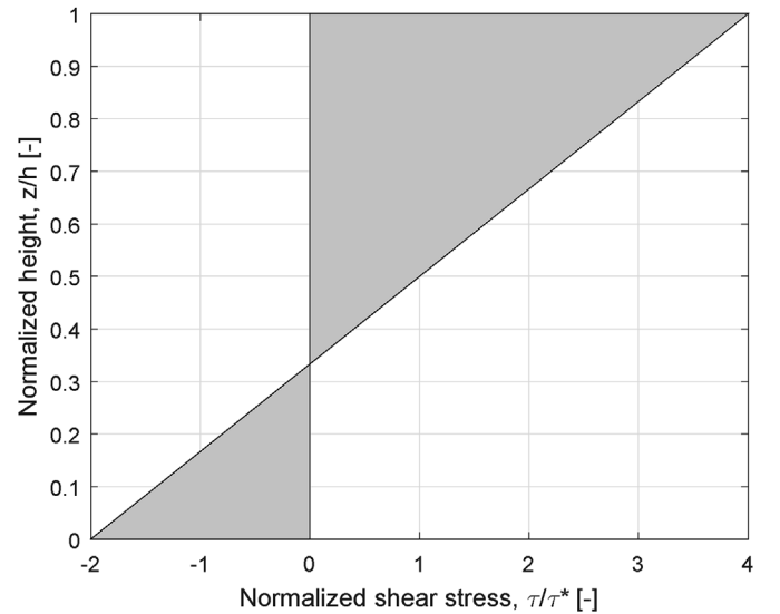
Fig. 4. This figure presents the normalized shear stress profile in-between the two bearing surfaces of a ferrofluid bearing, as described in (18). The shear stress is normalized for \tau^* = \frac{\tau h}{\eta U} .
