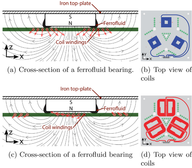
Fig. 6. The coils create a resultant out-of-plane (6a) and in-plane (6c) force as a result of the Lorentz forces and designed coil configuration. Fig. 6d and b shows the coil configuration from a top-view, with the three coil-sets corresponding to three ferrofluid bearings.
