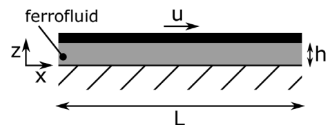
Fig. 2. Two large plates ( L \gg h ) moving with respect to each other with velocity u and separated with a ferrofluid film with height h .
