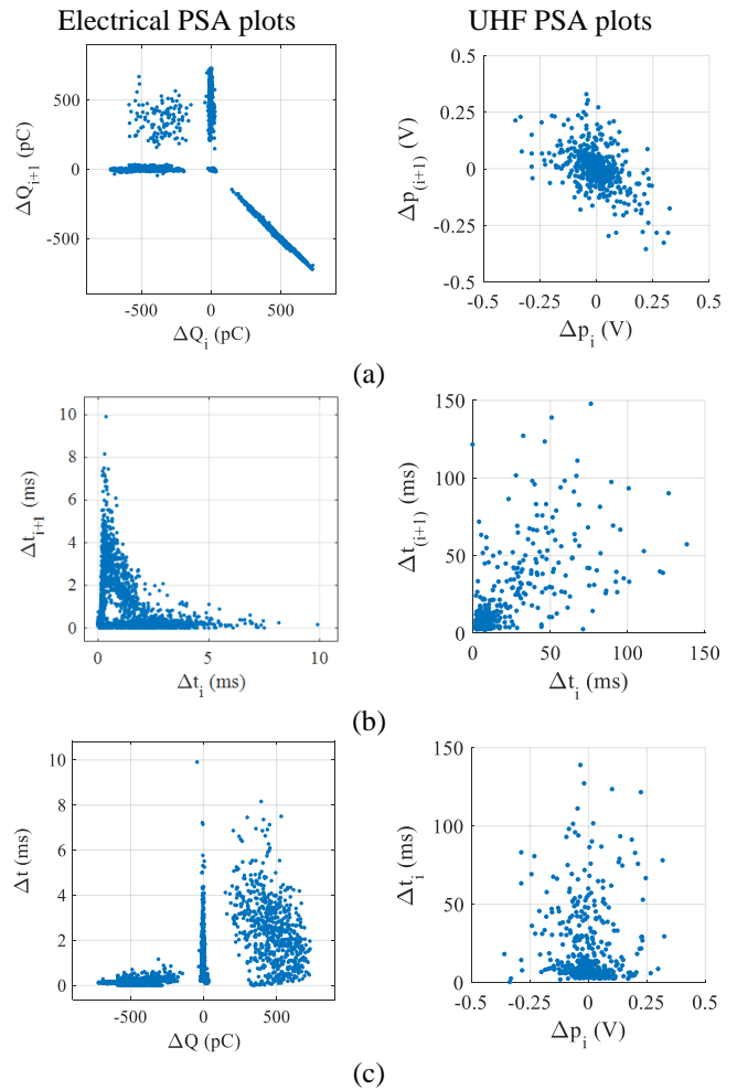
Fig. 7. PSA pattern of floating nut electrode at V_{DC} = -27.7 kV; a) correlation of difference in amplitude; b) correlation of difference in time delay; c) correlation of difference in time delay and amplitude
