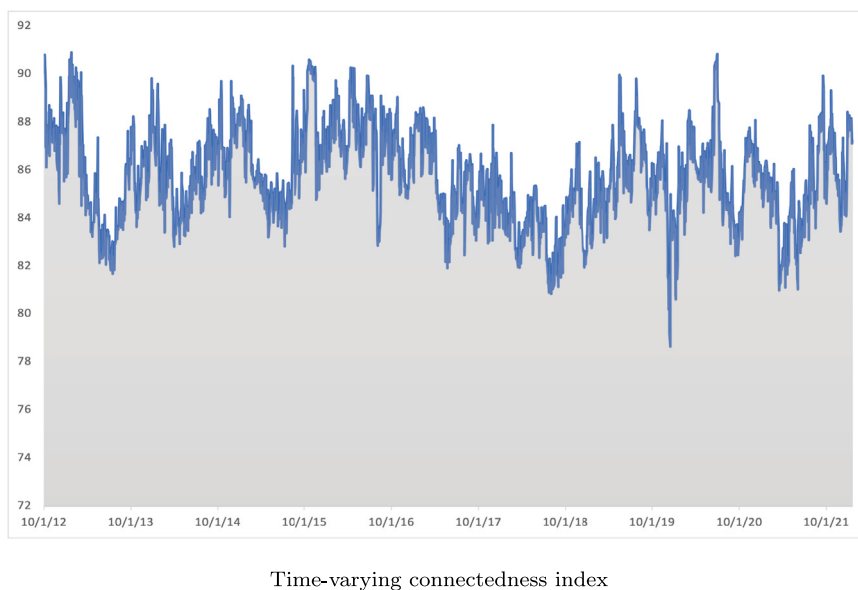
Fig. 7. Time-varying connectedness for the quantile VAR (upper quantile - \tau_{0.95} ).
