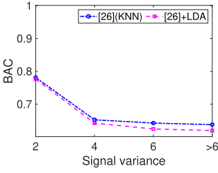
Fig. 16. LDA contribution.
