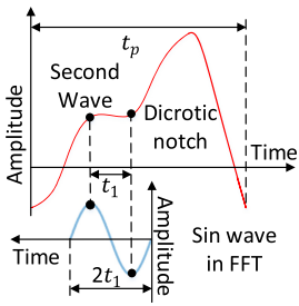
Fig. 5. Frequency analysis to determine the upper cut-off frequency f_h .
