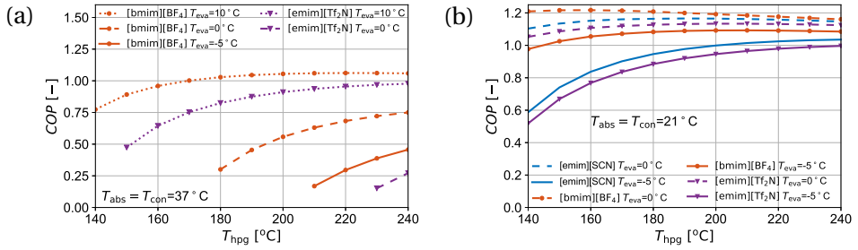
Figure 7.13: Influence of cooling temperature, T_{eva} , on the coefficient of performance of the DE-VAR cycle with working pairs \text{NH}_3/[\text{emim}][\text{SCN}] (smooth curves), \text{NH}_3/[\text{bmim}][\text{BF}_4] (●) and \text{NH}_3/[\text{emim}][\text{Tf}_2\text{N}] (▼) for applications in: (a) tropical areas ( T_{con} = T_{abs} = 37^\circ\text{C} ) and (b) high-latitude areas ( T_{con} = T_{abs} = 21^\circ\text{C} ).
