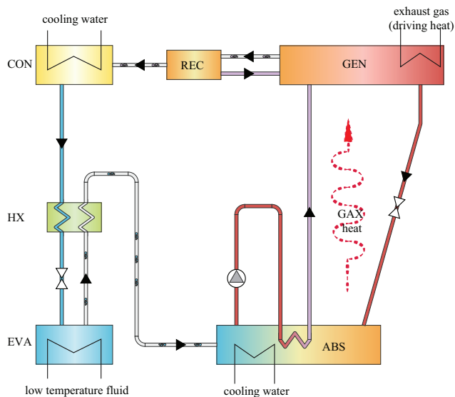
Figure 7.7: Schematic diagram of a standard \text{NH}_3/\text{H}_2\text{O} GAX cycle [327]. The main feature of the GAX cycle is that the final stages of its ABS have higher temperatures than the flow in the first stages of the GEN. The heat from the ABS is recycled to heat up later stages in the GEN. The weak \text{NH}_3/\text{H}_2\text{O} solutions absorb \text{NH}_3 vapors from the EVA and experience an internal heat recycling in the ABS before they are pumped into the GEN. Vapors leaving the GEN are mixtures of \text{NH}_3/\text{H}_2\text{O} , which are purified in the rectifier (REC). \text{NH}_3 vapor is treated similarly as in the DE-VAR cycle to generate the cooling effect.
