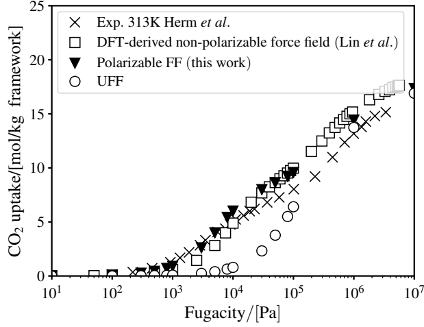
Figure 2.6: Comparison between the experimental adsorption isotherm of CO 2 in Mg-MOF-74 from Herm et al. [20] and the ones predicted from molecular simulation at 313 K. The UFF force field [72] cannot reproduce the inflection of the adsorption isotherm and the CO 2 uptake in the low pressures region. The force field previously developed by Lin et al. (model 3) [80] derived from DFT calculations can capture the adsorption. The simulations conducted with polarizable force field are in good agreement with the experimental results. The low pressure region and the inflection of the adsorption isotherm are well modeled. The used scaling factor \lambda for the Lennard-Jones potential is 0.7. The atomic polarizabilities are from van Duijnen and Swart, and Shannon [218, 219] and scaled with a factor of 0.09.
