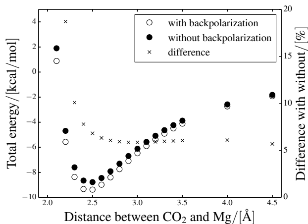
Figure 2.2: Total energy of a single \text{CO}_2 molecule in Mg-MOF-74 calculated using the developed polarizable force field as a function of the distance to the open metal site. Comparison between interactions with and without back-polarization.
