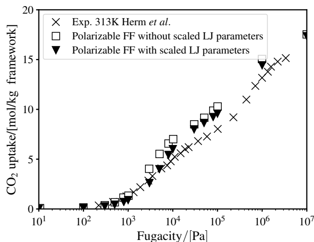
Figure 2.4: Comparison between the experimental adsorption isotherm of \text{CO}_2 in Mg-MOF-74 from Herm et al. [20] and the simulated ones using polarizable force fields at 313 K. In both simulations, the atomic polarizabilities are taken from van Duijnen and Swart, and Shannon [218, 219] and scaled with a factor of 0.09. The open squares represent the simulation results using the non-scaled Lennard-Jones potential. The adsorption isotherm shown by closed triangles is calculated with a scaling factor \lambda = 0.7 for the Lennard-Jones potential. In case of adjusted Lennard-Jones parameters, simulation results are in better agreement with experiments.
