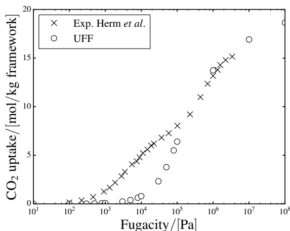
Figure 1.2: Comparison between the experimental adsorption isotherm of CO 2 in Mg-MOF-74 from Herm et al. [20] and the simulated one using the UFF force field [72] for Mg-MOF-74 and the TraPPE force field [73] for CO 2 at 313 K.
