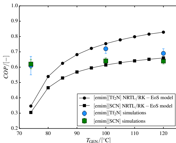
Figure 6.6: Comparison between the COP calculated from simulations (colored) and from the NRTL/EoS model (black) for [emim][Tf 2 N] (●) and [emim][SCN] (■). The cycle conditions in this work are: T_{\text{CON}} = 35^{\circ}\text{C} , T_{\text{ABS}} = 30^{\circ}\text{C} , T_{\text{EVA}} = 10^{\circ}\text{C} , T_{\text{GEN}} = 74\text{--}120^{\circ}\text{C} , P_{\text{EVA}} = 6.15\text{ bar} , and P_{\text{CON}} = 13.5\text{ bar} .
