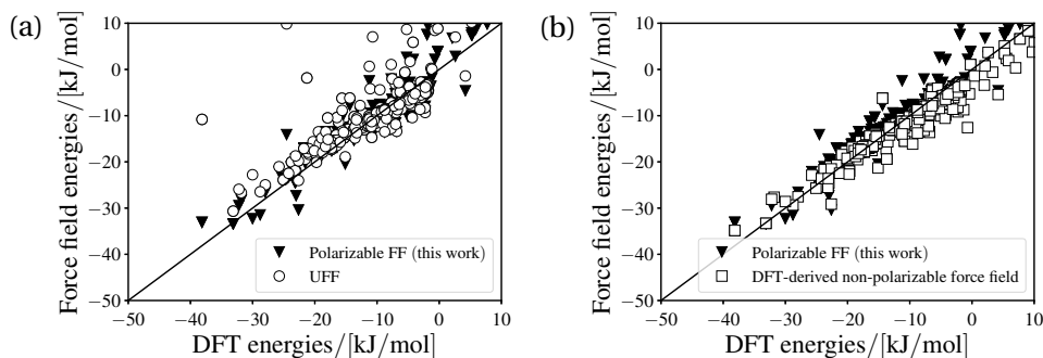
Figure 2.5: \text{CO}_2 -framework interaction energies for a set of 600 randomly located \text{CO}_2 configurations in the accessible volume of Mg-MOF-74. Interaction energies computed in DFT calculations are from Lin et al. [80]. The solid line indicates perfect agreement between the force field and DFT energies. (a) Comparison between the polarizable force field and the UFF force field [72]. (b) Comparison between the polarizable force field and the DFT-derived non-polarizable force field of Lin et al. (model 3) [80].
