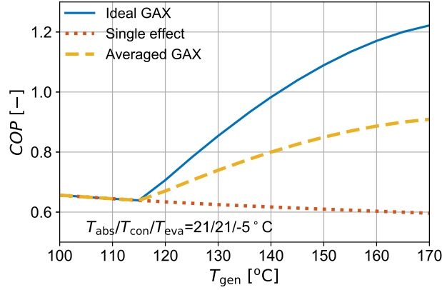
Figure 7.14: Comparison of the performance between the ideal \text{NH}_3/\text{H}_2\text{O} GAX cycle and the single-stage \text{NH}_3/\text{H}_2\text{O} cycle at various T_{\text{gen}} ( T_{\text{abs}}/T_{\text{con}}/T_{\text{eva}} = 21/21/-5^\circ\text{C} ). The solid curve indicates the “ideal” GAX performance and the dotted curve indicates the “degraded” GAX, i.e., the SE cycle. The dashed curve denotes the estimated performance of a real system.
