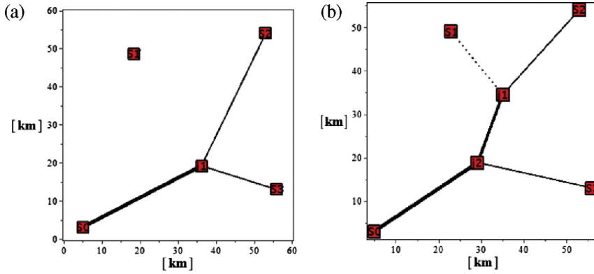
Fig. 5. Network layout concepts based on design strategy 1 (a) and design strategy 2 (b).
