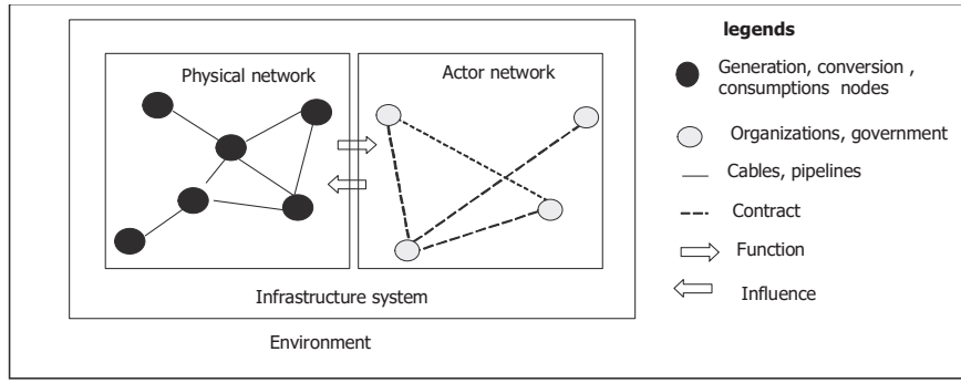
Figure 2.1 Abstraction of energy and industrial infrastructures as networks of physical artefacts and networks of actors.
