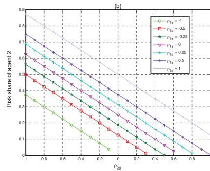
Fig. 1. Optimal risk share as function of correlation coefficients: (a) agent 1, and (b) agent 2.
