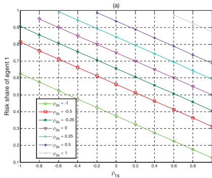
Fig. 1. Optimal risk share as function of correlation coefficients: (a) agent 1, and (b) agent 2.
