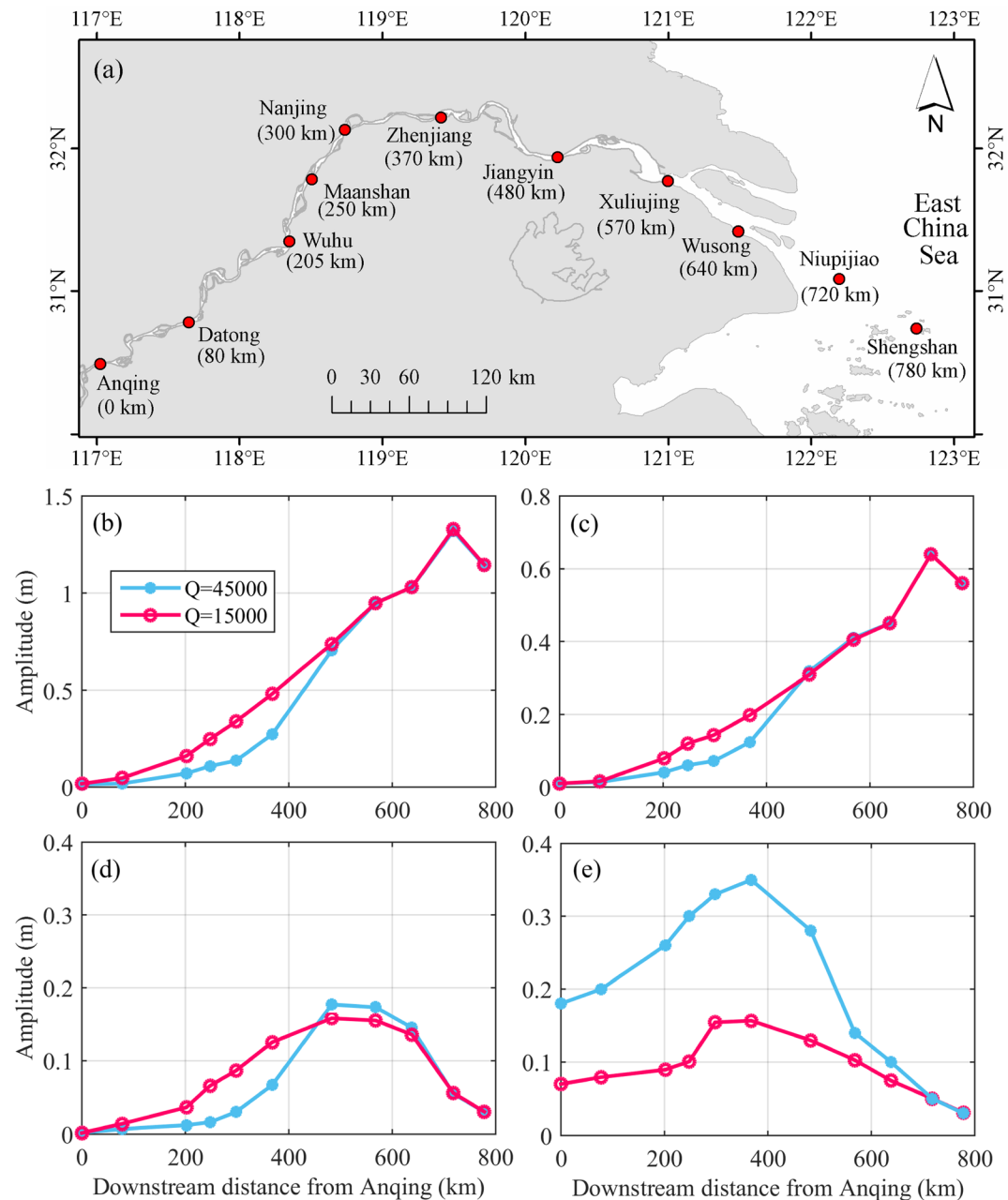
Figure 1. (a) Map of the Changjiang Estuary showing the location of the tidal gauges and along-river variations of the tidal amplitudes of (b) M_2 , (c) S_2 , (d) MS_4 , and (e) MS_f in the wet and dry seasons when the mean river discharge is \sim 45,000 and \sim 15,000 \text{ m}^3/\text{s} , respectively. A description of the Changjiang Estuary is provided in Guo et al. (2015). The numbers in the brackets in panel (a) indicate that the seaward distance from Anqing River discharge was traditionally monitored at Datong, the tidal wave limit, while water level data at Anqing are included in this work to demonstrate more inland tidal influence.
