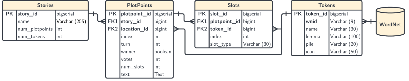
Figure 4: TaleMaker's Database Schema
