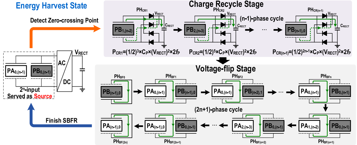
Fig. 11. Structure transformation of 2^n -input array in zero-crossing state of the proposed SBFR_z .
