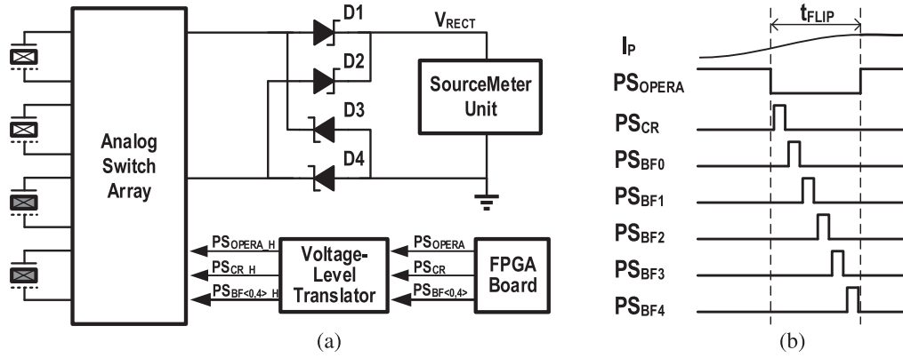
Fig. 13. Principle of the test. (a) Test bench schematic. (b) Control signal.
