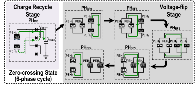
Fig. 6. Zero-crossing state of the SBF_4 .
