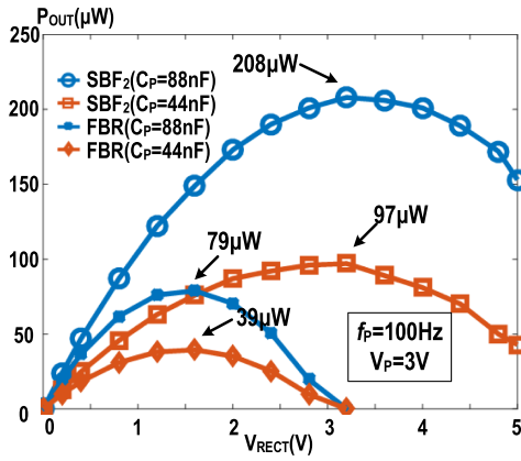
Fig. 16. Measured effect of C_P area on harvested power with SBF 2 and FBR.
