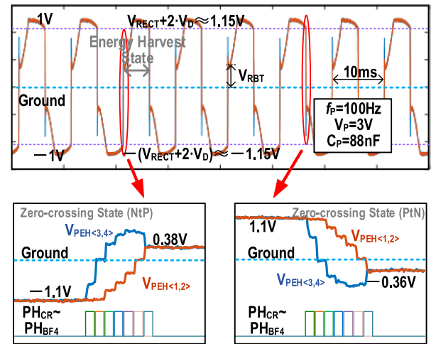
Fig. 18. Measured waveform of the V_{PEH} with SBF 4 .
