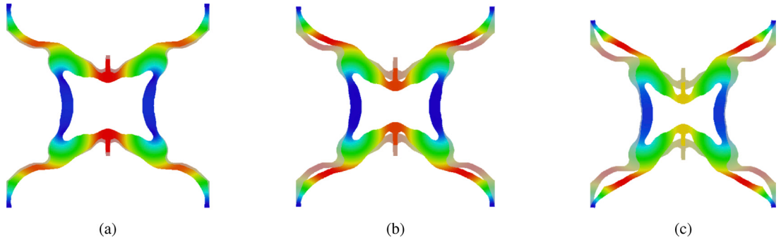
Fig. 21. Deformed profiles of the contractor CM at different pressure loads. CT3 Pa-CMs (a) 10 bar, (b) 25 bar, (c) 50 bar.
