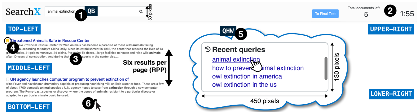
Figure 3: The SearchX search interface used for this study. Note the inclusion of the QHW in the callout—this was positioned in one of the areas as shown with blue boxes. Refer to §5.2 for information on the circled interface components.
