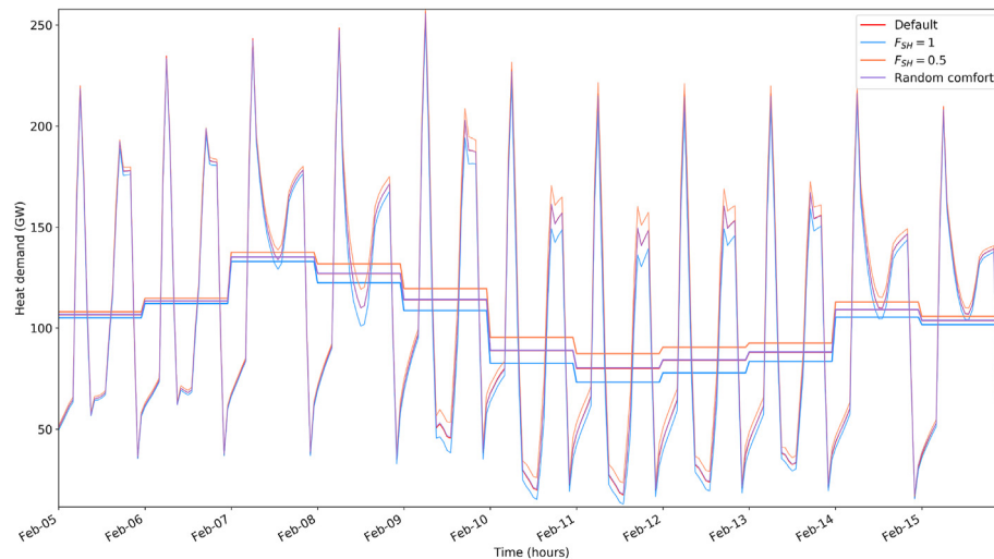
Fig. 7. Sensitivity of model results to variations of uncertain parameters for a representative 10-day period in February (2015 weather data). The figure shows both the hourly profiles and the daily average heat demand for Italy as a whole, for each sensitivity scenario and for the default model settings.
