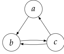
Figure 4.2: A graph with a transitive elimination ordering (a, b, c)
