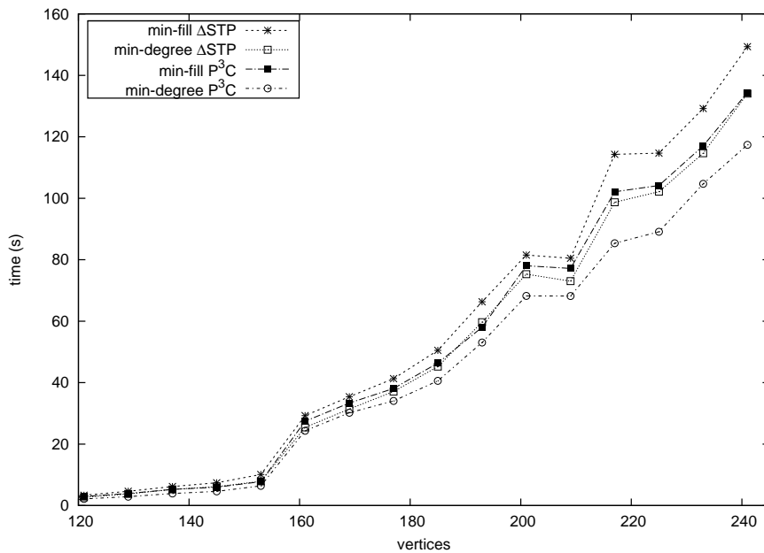
Figure 6.13: Enforcing PPC for job shop (large instances)
