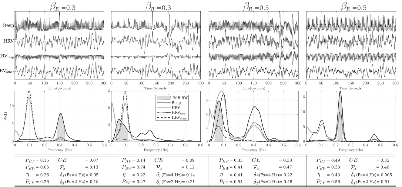
Fig. 5. Examples of signals in the simulation study with different respiratory signals and \beta_R . Top row: Signals and HRV decomposition with subspace projections. Middle row: PSD estimates of the signals. The gray region corresponds to the -3 dB bandwidth of the respiration. Bottom row: RSA strength estimated with the approaches included in this paper. Two examples with \beta_R = 0.3 and two examples with \beta_R = 0.5 are illustrated to show the response of the RSA estimates to respirations with different spectral characteristics but with modulating signals with the same \beta_R .
