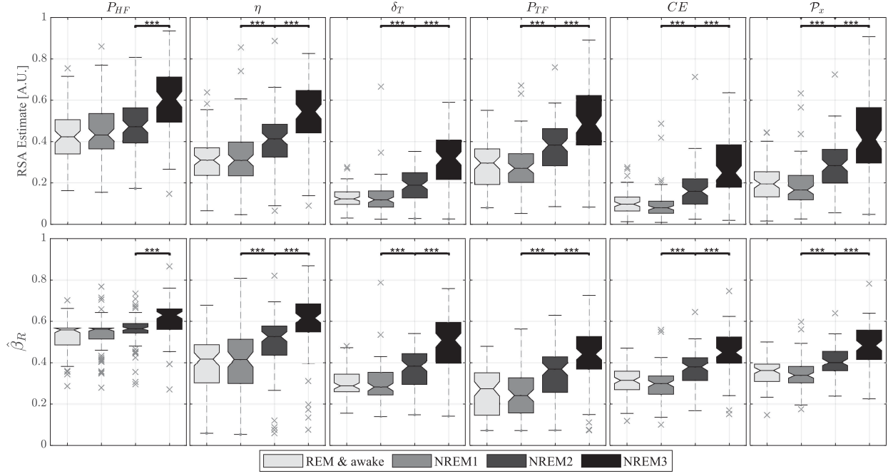
Fig. 9. RSA changes in the sleep dataset. Top row: RSA estimates with the approaches compared in this paper. Each estimate measures the RSA in a different unit and/or scale: \eta \in [0 \infty] and is given in s^{-1} ; CE \in [0 \infty] and is unit less; P_{HF} , \delta_T , P_{TF} and P_x \in [0 1] and are given as ratios, but each of them correlates differently to the RSA. Bottom row: equivalent \hat{\beta}_R for each RSA estimate after using the SVM regression models. \hat{\beta}_R \in [0 1] and is the proportion of variance due to the respiratory component in the modulating signal. Significant differences between sleep stages were tested with Friedman's test for repeated measures.
