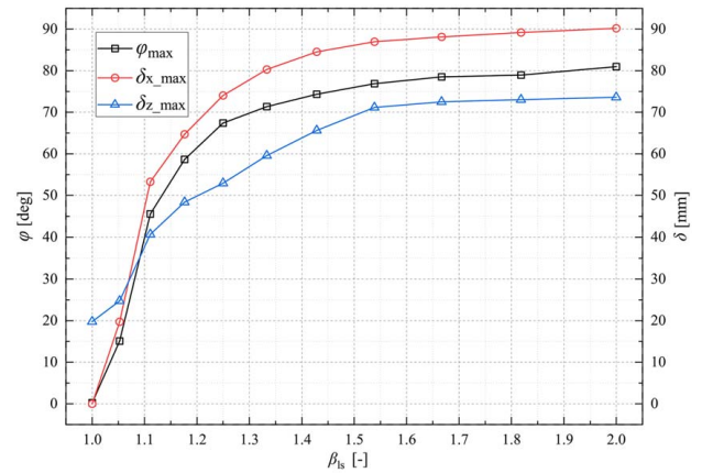
Fig. 18 The actuator bending angle and deflection curves of different \beta_{1s}
