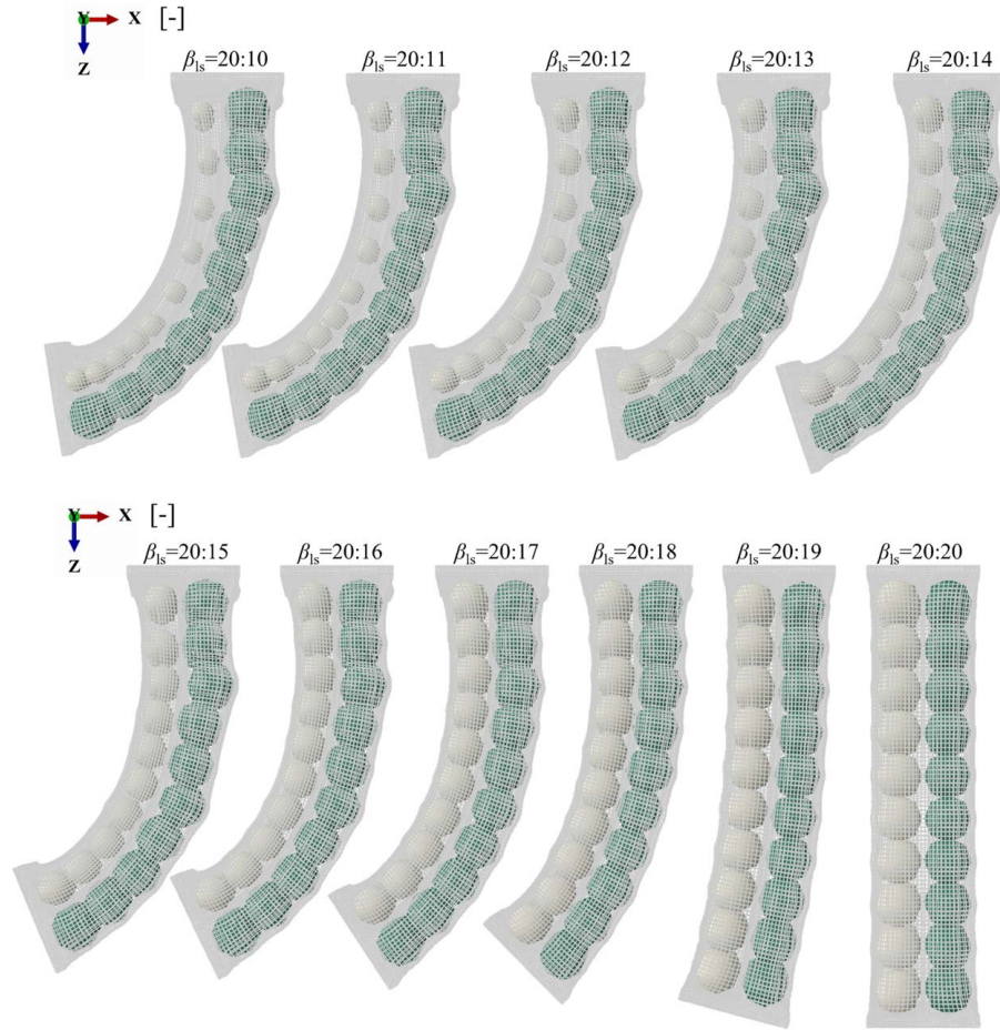
Fig. 17 The actuator bending performance of different \beta_{1s}
