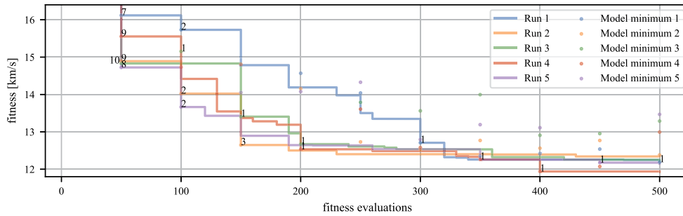
Figure 12. Pretrained individual transfer surrogate applied to the Dawn problem (Pop. 10, Gen. 5, Seq. 10)
