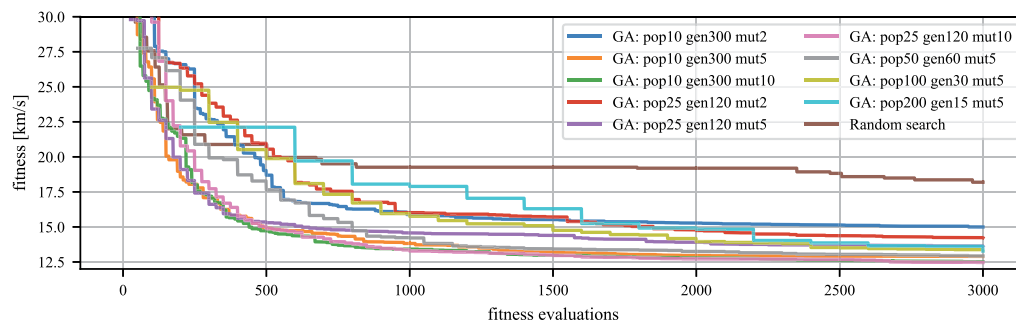
Figure 5. Comparison of different GA settings for population size and mutation probability, average of 5 runs each, optimizing the Dawn Problem
