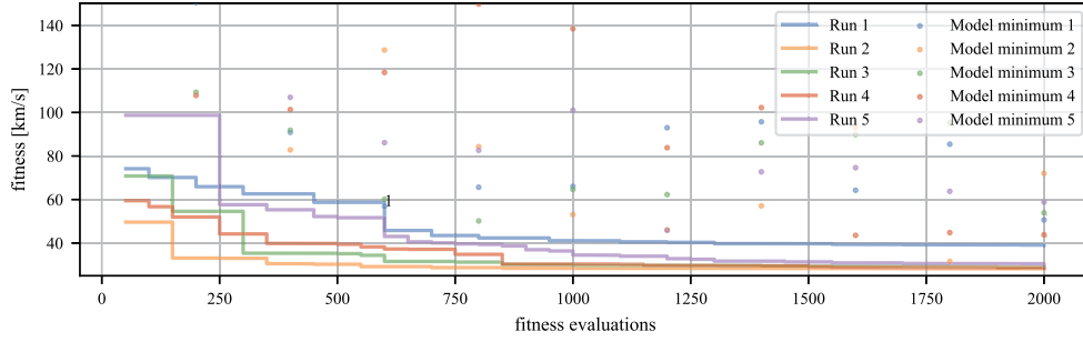
Figure 15. Full surrogate applied to the Asteroid problem (Pop. 50, Gen. 4, Seq. 10)
