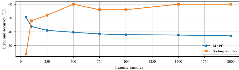
Figure 2. Regression accuracy of a linear regression model
