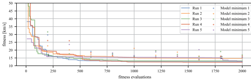
Figure 11. Individual transfer surrogate applied to the Dawn problem (Pop. 10, Gen. 20, Seq. 10)
