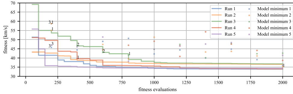
Figure 17. Individual transfer surrogate applied to the Asteroid problem (Pop. 50, Gen. 4, Seq. 10)
