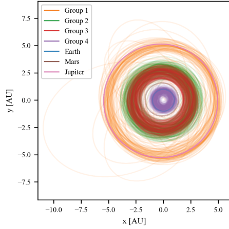
Figure 13. The GTOC2 asteroids
