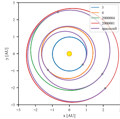
Figure 8. Optimized Dawn problem
