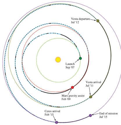
Figure 7. The trajectory of the Dawn mission 26
