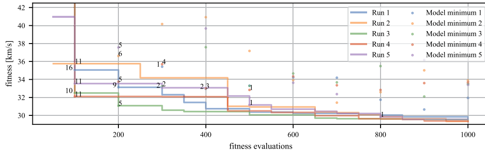
Figure 18. Pretrained general transfer surrogate applied to the Asteroid problem (Pop. 50, Gen. 2, Seq. 10)
