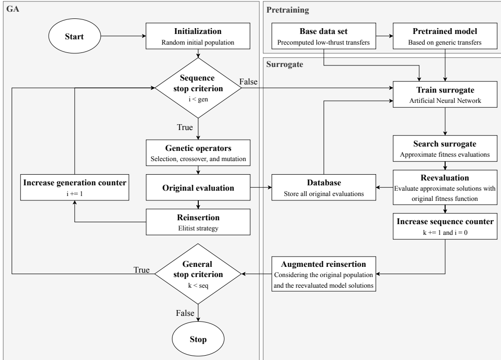
Figure 6. The augmented GA using an ANN surrogate to find new candidate solutions
