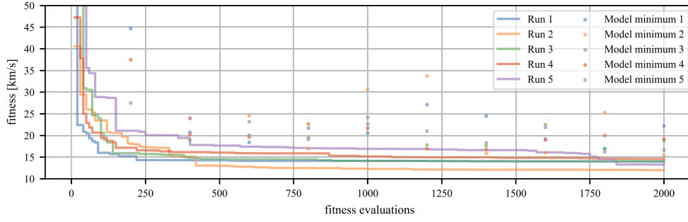
Figure 9. Full surrogate applied to the Dawn problem (Pop. 10, Gen. 20, Seq. 10)
