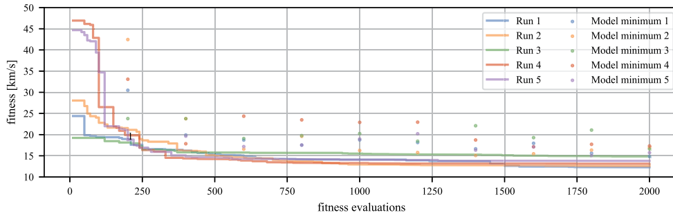
Figure 10. General transfer surrogate applied to the Dawn problem (Pop. 10, Gen. 20, Seq. 10)
