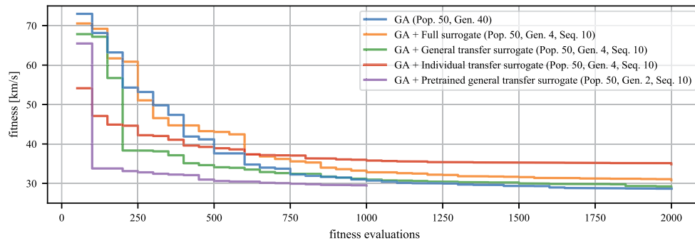
Figure 20. Averaged convergence of the investigated algorithms on the Asteroid problem
