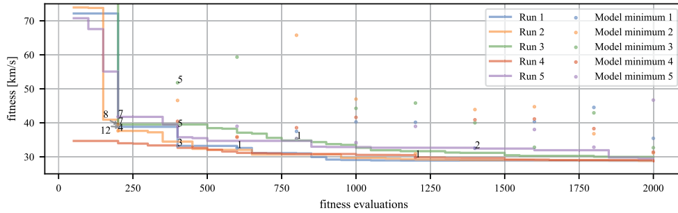
Figure 16. General transfer surrogate applied to the Asteroid problem (Pop. 50, Gen. 4, Seq. 10)
