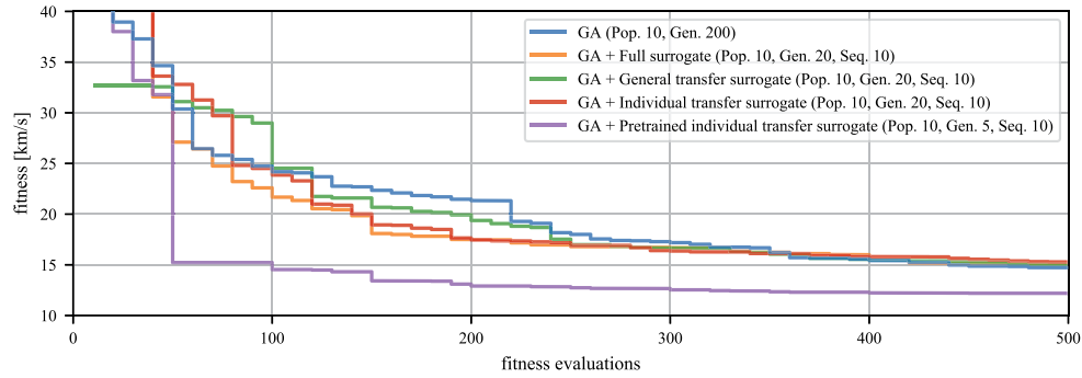
Figure 19. Averaged convergence of the investigated algorithms on the Dawn problem
