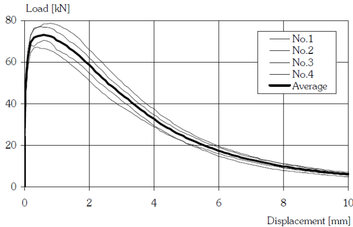
Figure 4: Flexural results and average of four prisms produced with SCC containing 125 \text{ kg/m}^3 steel fibres.
