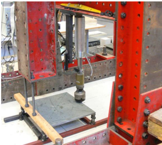
Figure 6: The testing machine with a thin plate placed on four supports; the loading head is placed between two supports at the edge of the plate.
