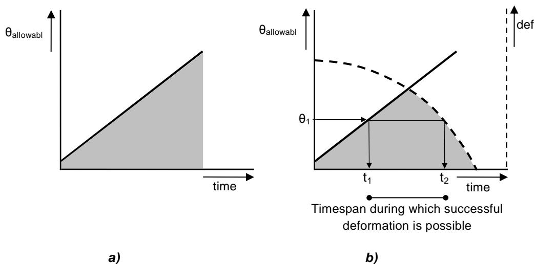
Figure 3: Increase of yield strength of concrete in time (a) and decrease of deformability and timespan to deform the mould (b) [9].
