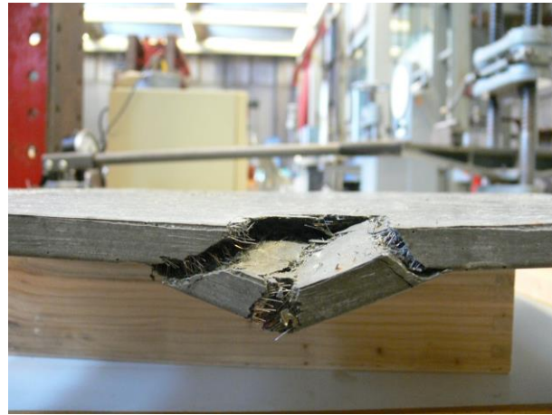
Figure 9b: Horizontal view on Plate 6 after the execution of the test.
