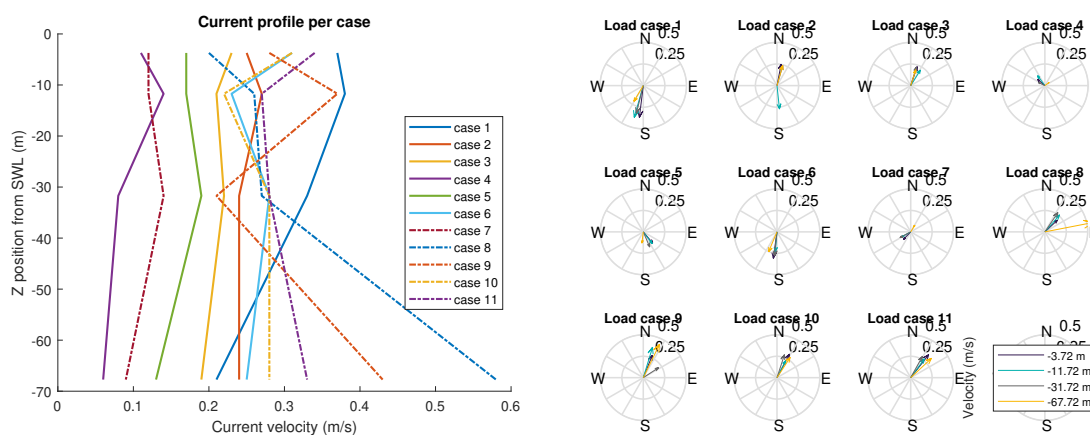
(a) Current profile for each load case.
