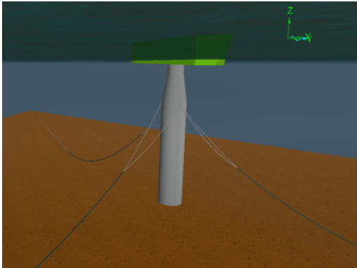
(a) BHawC/OrcaFlex model of the Hywind Scotland floating offshore wind turbine in shaded graphics view.
