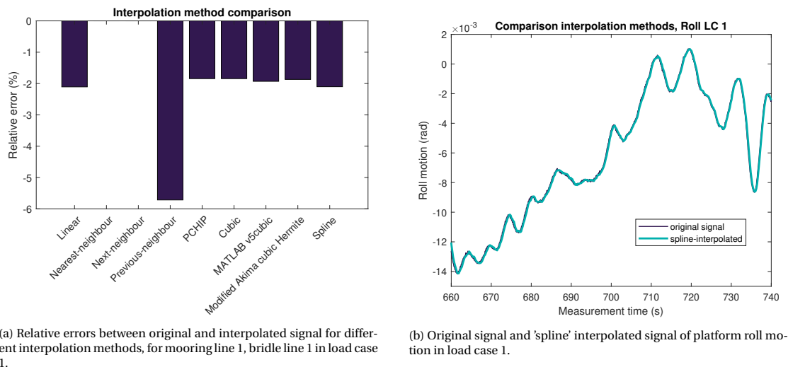
Figure E.1: An example of the effect of interpolation on the Hywind measurement signals.
