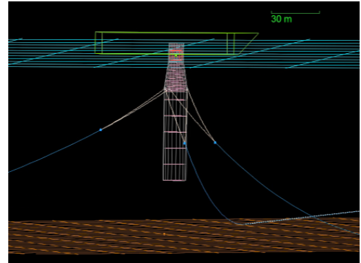
(b) BHawC/OrcaFlex model of the Hywind Scotland floating offshore wind turbine in wired frame view.
