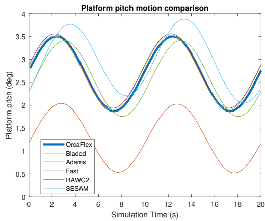
(c) Platform pitch motion.
