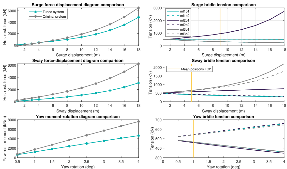
(a) Force-displacement diagram for surge and sway and moment-rotation diagram for yaw DOF of the tuned and un-tuned mooring system. (b) Bridle line tension for given surge, sway and yaw displacement of the tuned mooring system.
