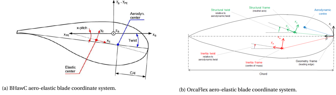
Figure 4.2: Overview of the blade section coordinate systems used in BHawC and in OrcaFlex. The steps for rewriting BHawC coordinates to OrcaFlex coordinates can be found in C.1
