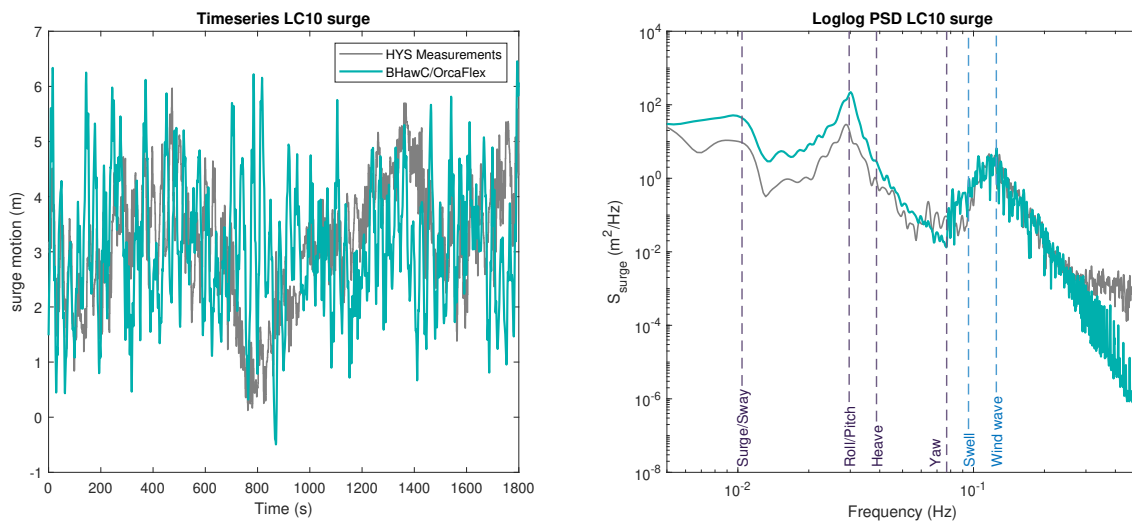
Figure 5.23: Comparison of platform surge response of load case 10 predicted by BH/OF and full-scale measurements.
