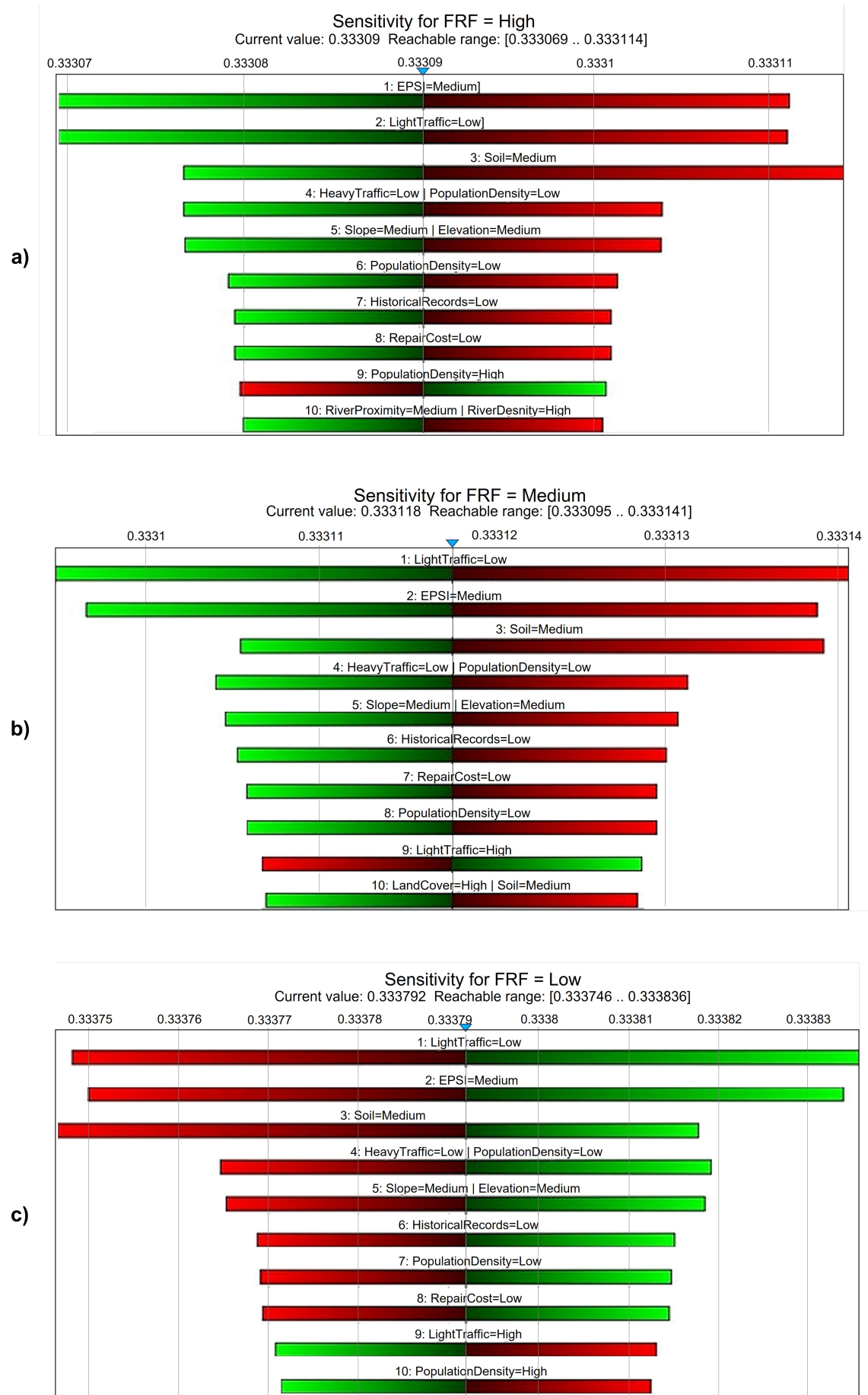
FIGURE 7. FRF Sensitivity Analysis: a) High, b) Medium and c) Low.
