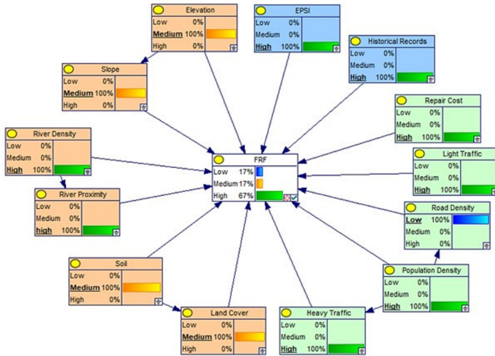
FIGURE 8. BN analysis FRF results of Vala da Azambuja road network .
