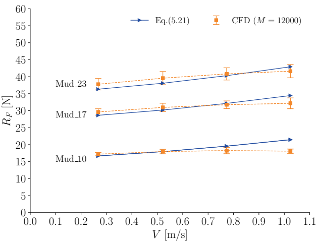
Figure 5.23: Comparison of the frictional resistance obtained with Eq. (5.21) and CFD using large regularisation parameters ( M = 12000 ).
