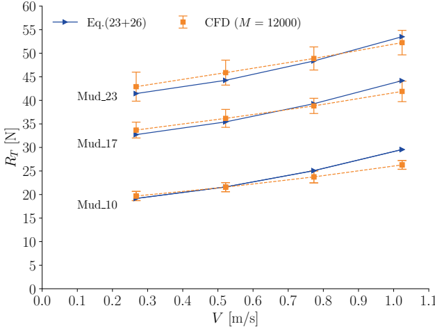
Figure 5.26: Comparison of the total resistance predicted by analytical formulas and CFD data.
