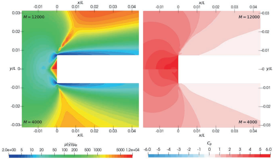
Figure 5.10: Effect of regularisation parameter M on the apparent viscosity (left) and pressure coefficient (right) at the leading face of the plate for Mud_23 and V = 0.27 m/s. Viscosity is in logarithmic scale. Flow is from left to right. The cutting plane is at z/T = -0.5 .
