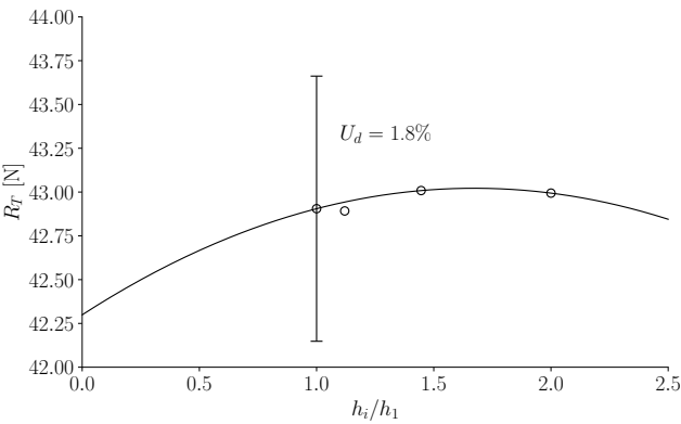
Figure 5.8: Grid sensitivity of R_T for Mud_23, V = 0.27 m/s. The grid refinement ratios are h_i/h_1 = 1, 1.12, 1.45, 2 , which correspond to grids having 1.77, 1.26, 0.59, 0.22 millions cells, respectively,.
