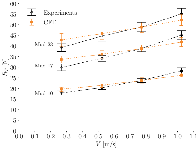
Figure 5.11: Total resistance of the plate moving through mud as a function of the inflow velocity. CFD error bars include numerical and input parameter uncertainties. CFD data were obtained keeping the non-dimensional regularisation parameter at M = 12000 (see also Section 5.3.4).
