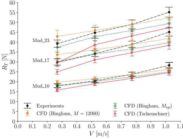
Figure 5.18: Total resistance using the Bingham and Tscheuschner model. The Tscheuschner uncertainty bars are set to 5% as a reference.
