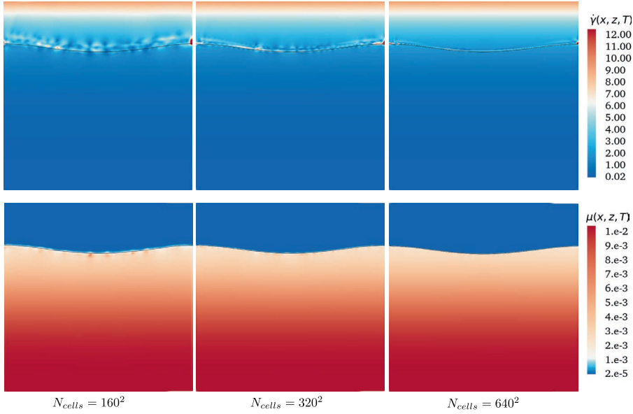
Figure 3.9: Contour plots of the shear rate \dot{\gamma} [ \text{s}^{-1} ] (top panel) and the viscosity \mu(\dot{\gamma}) [Pa s] (bottom panel) for different refinement levels at computational time t = T . The artefacts caused by spurious velocities are clearly visible near the free surface on the grid with 160^2 cells.
