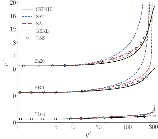
Figure 6.6: Average viscosity for Re_\tau = 323 . DNS data are from Singh et al. [153].
