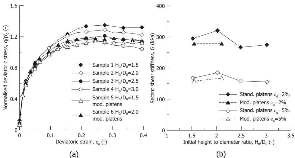
Figure 3.3: Deviatoric stress-strain response (a) and secant shear stiffness (b) upon undrained compression tests on samples with different height to diameter ratio tested with standard and modified end platens
