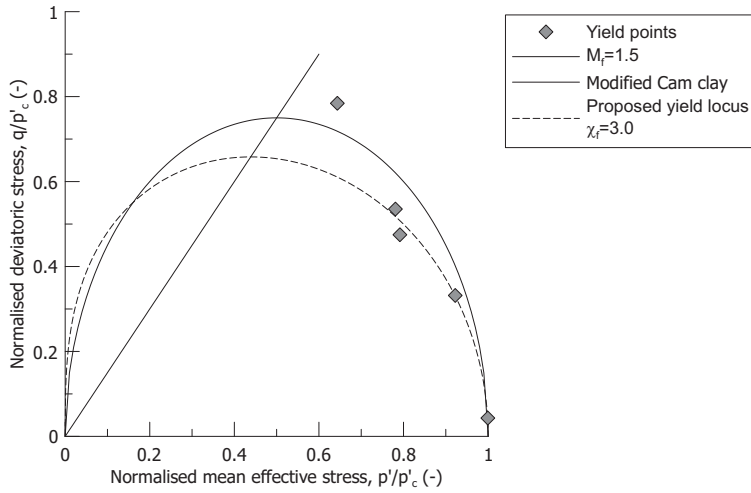
Figure 5.5: Trace of the yield locus on the p' - q space from the estimated yield points
