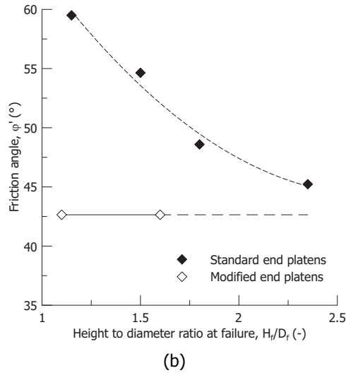
Figure 3.10: Stress ratio plotted against deviatoric stress rate (a) and (b) friction angle estimated from undrained compression tests on samples with different height to diameter ratio tested with standard and modified end platens
