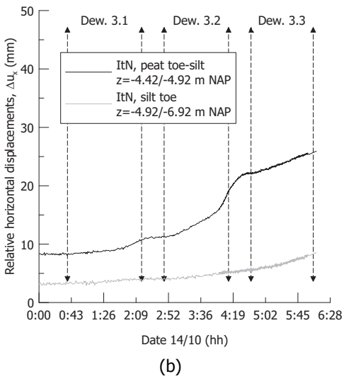
Figure 2.21: Horizontal displacements recorded by the inclinometer ItN at the toe of the dyke (a) and (b) relative horizontal displacements recorded at different depths during October 14 from the inclinometer ItN
