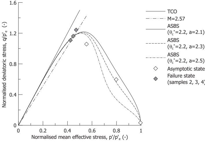
Figure A.3: Asymptotic state boundary surface used in the model compared to the experimental data
