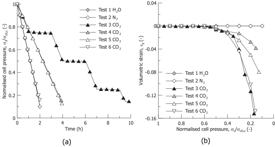
Figure 7.2: Undrained unloading stage: (a) normalised cell pressure time sequence, (b) volumetric strains
