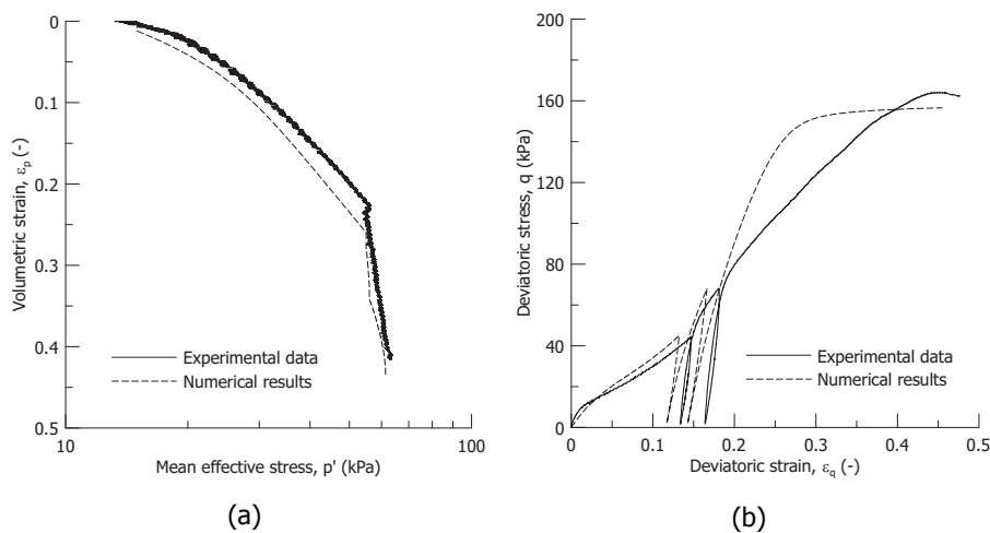
Figure A.8: Comparison between the experimental results and the model simulations for sample 2 in terms of (a) volumetric response and (b) deviatoric response
