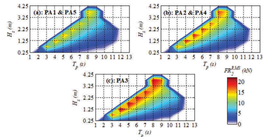
Figure 18. FR_2^{qRMS} , q=1, \dots, 5 , contours for equally-spaced arrays at S2.
