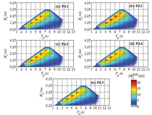
Figure 13. FR_2^{qRMS} , q=1, \dots, 5 , contours for optimally-arranged array at S1.
