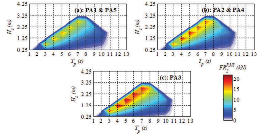
Figure 17. FR_2^{qRMS} , q=1, \dots, 5 , contours for equally-spaced arrays at S1.
