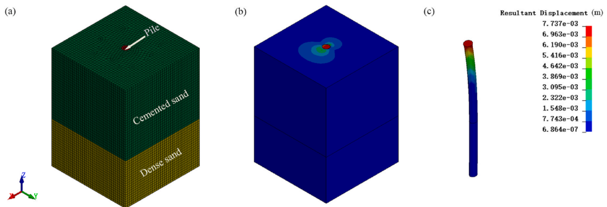
Fig. 6. Soil-structure interaction model (a) mesh configuration; (b) resultant displacement distribution with the external force of 100 kN in the x direction; (c) deflection of the pile in the soil.
