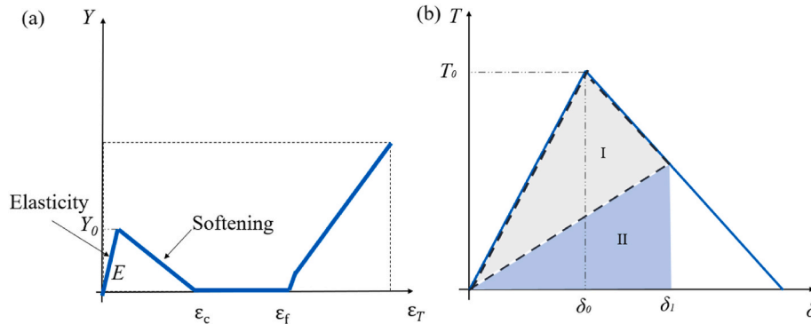
Fig. 1. Constitutive laws for (a) solid ice elements; (b) cohesive elements; where E is elastic modulus of the material; Y is stress; Y_0 is yield stress; \varepsilon_c is strain after the softening process; \varepsilon_f is failure strain; \varepsilon_T is true strain of bulk elements; \delta is the separation distance; \delta_0 is critical crack separation distance; \delta_I is failure separation distance; T represents traction; T_0 denotes the critical traction; Regions I and II represent the energy dissipation area.
