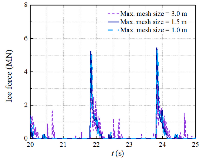
Fig. 4. Mesh sensitivity results.
